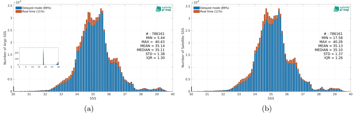
Figure 2: Histograms of SSS from Argo (a) and CCI SSS L4 Merged-OI v3.2 - 30-day running (ESA) (b) considering all match-up pairs per bins of 0.1 over the Mid-Low Latitudes 45N-45S Pi-MEP region and for the full satellite product period.
