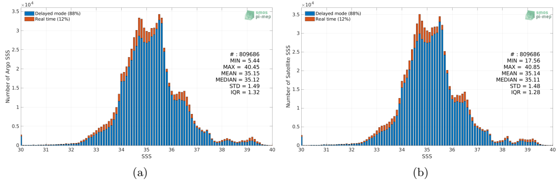
Figure 2: Histograms of SSS from Argo (a) and CCI SSS L4 Merged-OI v3.2 - 30-day running (ESA) (b) considering all match-up pairs per bins of 0.1 over the Mid-Low Latitudes 45N-45S Pi-MEP region and for the full satellite product period.
