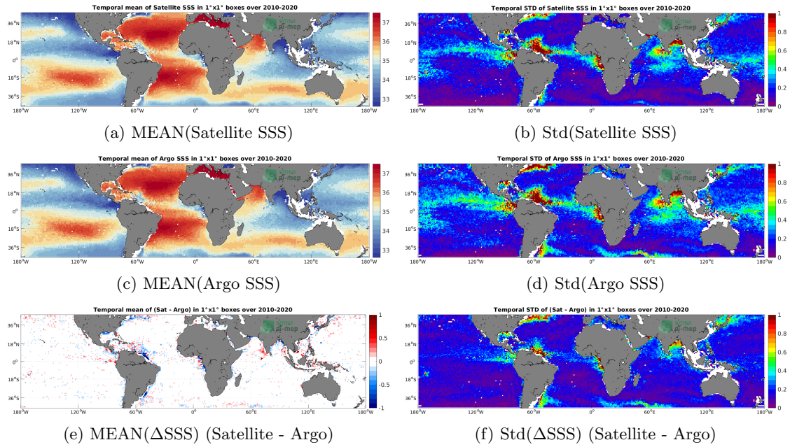
Figure 6: Temporal mean (left) and Std (right) of SSS from CCI SSS L4 Merged-OI v3.2 - 30-day running (ESA) (top), Argo (middle), and of \Delta SSS (Satellite - Argo). Only match-up pairs are used to generate these maps.
