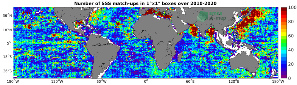
Figure 4: Number of SSS match-ups between Argo SSS and the CCI SSS L4 Merged-OI v3.2 - 30-day running (ESA) SSS product for the Mid-Low Latitudes 45N-45S Pi-MEP region over 1^\circ \times 1^\circ boxes and for the full satellite product period.
