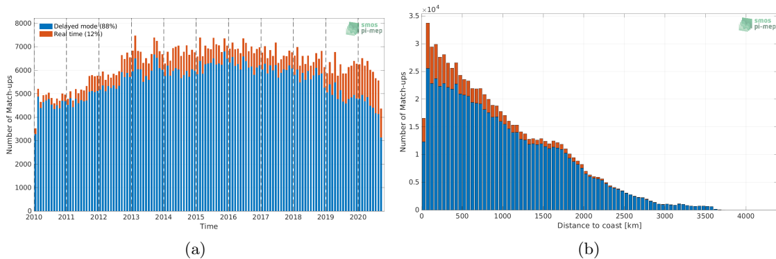
Figure 1: Number of match-ups between Argo and CCI SSS L4 Merged-OI v3.2 - 30-day running (ESA) SSS as a function of time (a) and as function of the distance to coast (b) over the Mid-Low Latitudes 45N-45S Pi-MEP region and for the full satellite product period.
