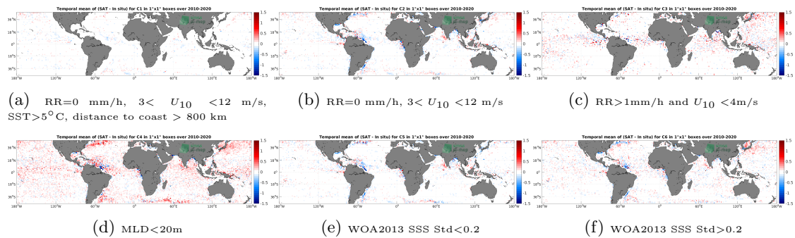
Figure 12: Temporal mean gridded over spatial boxes of size 1^\circ \times 1^\circ of \Delta SSS (CCI SSS L4 Merged-OI v3.2 - 30-day running (ESA) - Argo) for 6 different subdatasets corresponding to:RR=0 mm/h, 3 < U_{10} < 12 m/s, SST >5^\circ\text{C} , distance to coast > 800 km (a), RR=0 mm/h, 3 < U_{10} < 12 m/s (b), RR >1 mm/h and U_{10} < 4 m/s (c),MLD <20 m (d),WOA2013 SSS Std <0.2 (e),WOA2013 SSS Std >0.2 (f).
