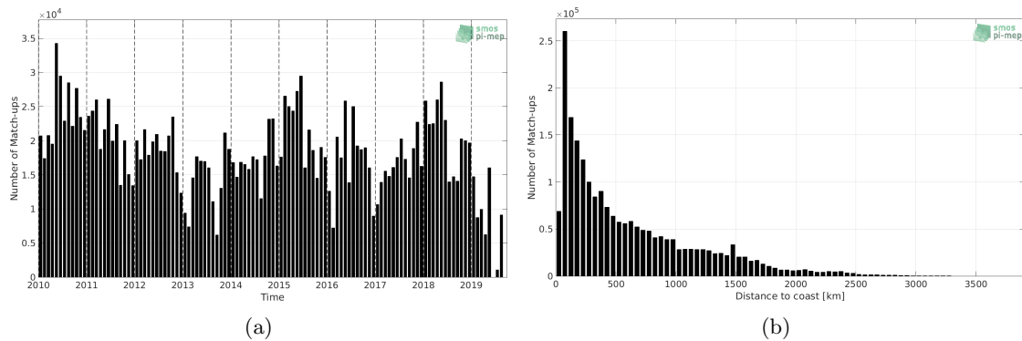
Figure 1: Number of match-ups between TSG (LEGOS-DM) and CCI SSS L4 Merged-OI v2.31 - 7-day running (ESA) SSS as a function of time (a) and as function of the distance to coast (b) over the Mid-Low Latitudes 45N-45S Pi-MEP region and for the full satellite product period.
