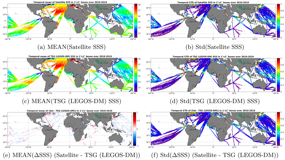
Figure 6: Temporal mean (left) and Std (right) of SSS from CCI SSS L4 Merged-OI v2.31 - 7-day running (ESA) (top), TSG (LEGOS-DM) (middle), and of \Delta SSS (Satellite - TSG (LEGOS-DM)). Only match-up pairs are used to generate these maps.
