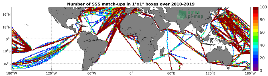
Figure 4: Number of SSS match-ups between TSG (LEGOS-DM) SSS and the CCI SSS L4 Merged-OI v2.31 - 7-day running (ESA) SSS product for the Mid-Low Latitudes 45N-45S Pi-MEP region over 1°x1° boxes and for the full satellite product period.
