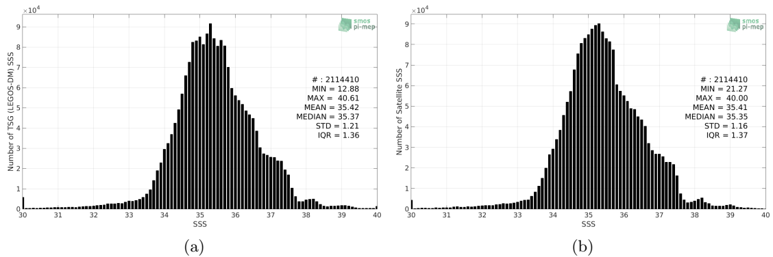
Figure 2: Histograms of SSS from TSG (LEGOS-DM) (a) and CCI SSS L4 Merged-OI v2.31 - 7-day running (ESA) (b) considering all match-up pairs per bins of 0.1 over the Mid-Low Latitudes 45N-45S Pi-MEP region and for the full satellite product period.
