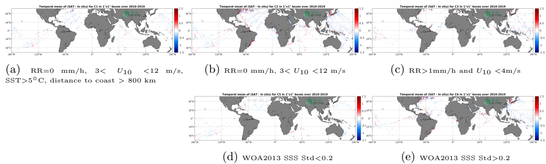
Figure 12: Temporal mean gridded over spatial boxes of size 1°x1° of \Delta SSS (CCI SSS L4 Merged-OI v2.31 - 7-day running (ESA) - TSG (LEGOS-DM)) for 5 different subdatasets corresponding to:RR=0 mm/h, 3 < U_{10} < 12 m/s, SST > 5°C, distance to coast > 800 km (a), RR=0 mm/h, 3 < U_{10} < 12 m/s (b), RR > 1mm/h and U_{10} < 4 m/s (c), WOA2013 SSS Std < 0.2 (d), WOA2013 SSS Std > 0.2 (e).
