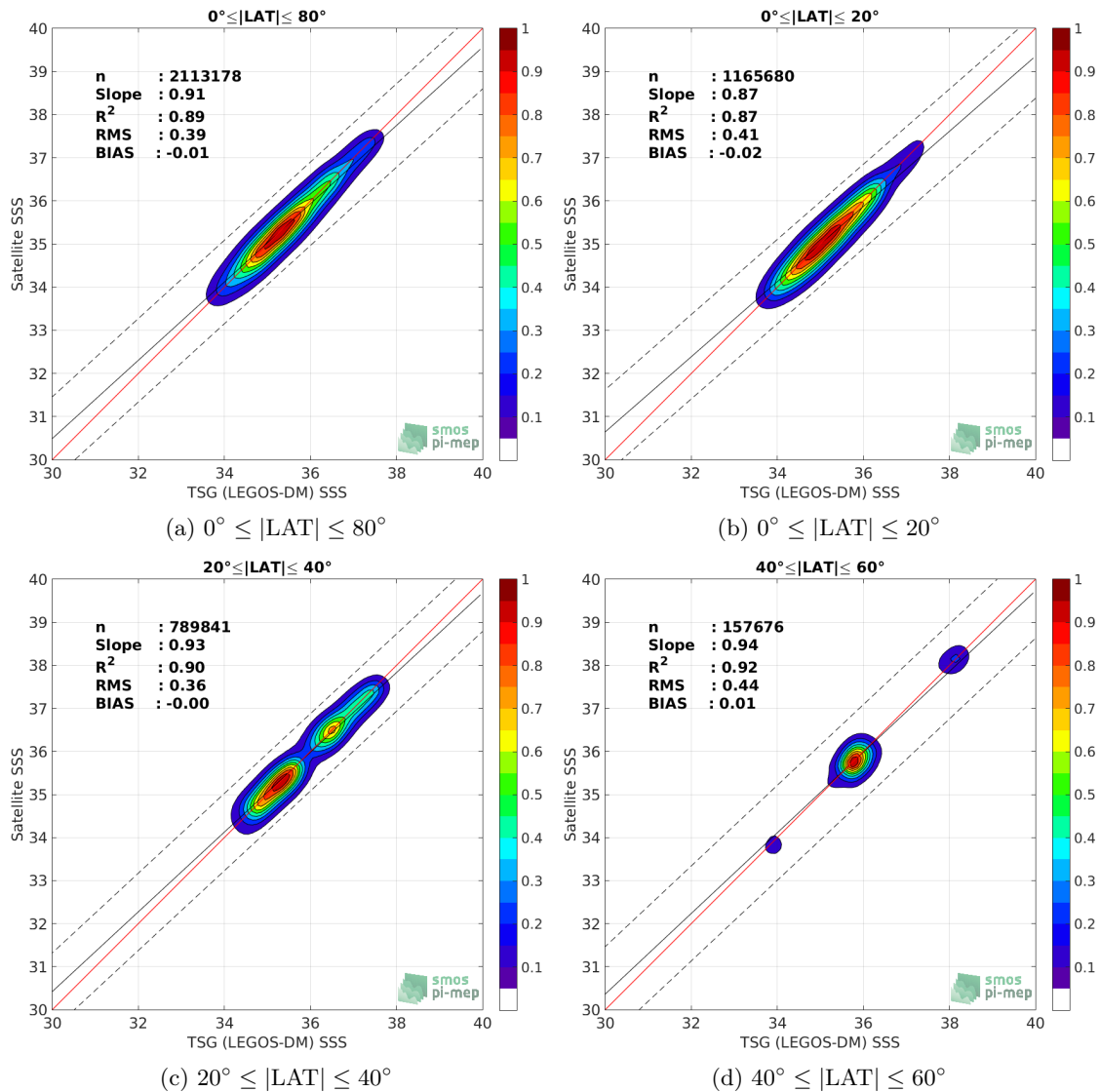
Figure 9: Contour maps of the concentration of CCI L4 Merged-OI v2.31 - 7-day running (ESA) SSS (y-axis) versus TSG (LEGOS-DM) SSS (x-axis) at match-up pairs for different latitude bands. For each plot, the red line shows x=y . The black thin and dashed lines indicate a linear fit through the data cloud and the \pm 95\% confidence levels, respectively. The number match-up pairs n , the slope and R^2 coefficient of the linear fit, the root mean square (RMS) and the mean bias between satellite and in situ data are indicated for each latitude band in each plots.
