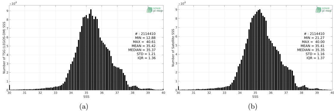
Figure 2: Histograms of SSS from TSG (LEGOS-DM) (a) and CCI L4 Merged-OI v2.31 - 7-day running (ESA) (b) considering all match-up pairs per bins of 0.1 over the Mid-Low Latitudes 45N-45S Pi-MEP region and for the full satellite product period.
