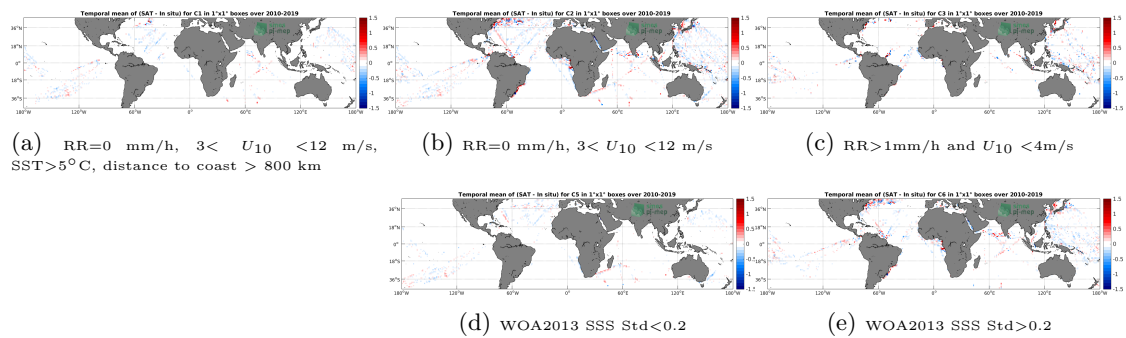
Figure 12: Temporal mean gridded over spatial boxes of size 1^\circ \times 1^\circ of \Delta SSS (CCI L4 Merged-OI v2.31 - 7-day running (ESA) - TSG (LEGOS-DM)) for 5 different subdatasets corresponding to: RR=0 mm/h, 3 < U_{10} < 12 m/s, SST > 5^\circ\text{C} , distance to coast > 800 km (a), RR=0 mm/h, 3 < U_{10} < 12 m/s (b), RR > 1 mm/h and U_{10} < 4 m/s (c), WOA2013 SSS Std < 0.2 (d), WOA2013 SSS Std > 0.2 (e).
