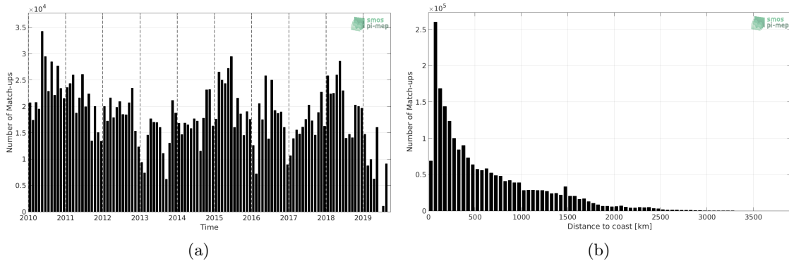
Figure 1: Number of match-ups between TSG (LEGOS-DM) and CCI L4 Merged-OI v2.31 - 7-day running (ESA) SSS as a function of time (a) and as function of the distance to coast (b) over the Mid-Low Latitudes 45N-45S Pi-MEP region and for the full satellite product period.
