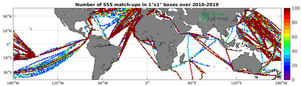
Figure 4: Number of SSS match-ups between TSG (LEGOS-DM) SSS and the CCI L4 Merged-OI v2.31 - 7-day running (ESA) SSS product for the Mid-Low Latitudes 45N-45S Pi-MEP region over 1°x1° boxes and for the full satellite product period.
