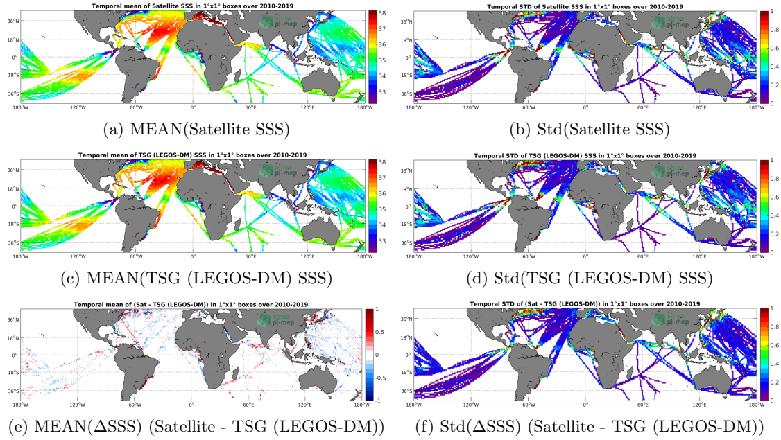
Figure 6: Temporal mean (left) and Std (right) of SSS from CCI L4 Merged-OI v2.31 - 7-day running (ESA) (top), TSG (LEGOS-DM) (middle), and of \Delta SSS (Satellite - TSG (LEGOS-DM)). Only match-up pairs are used to generate these maps.
