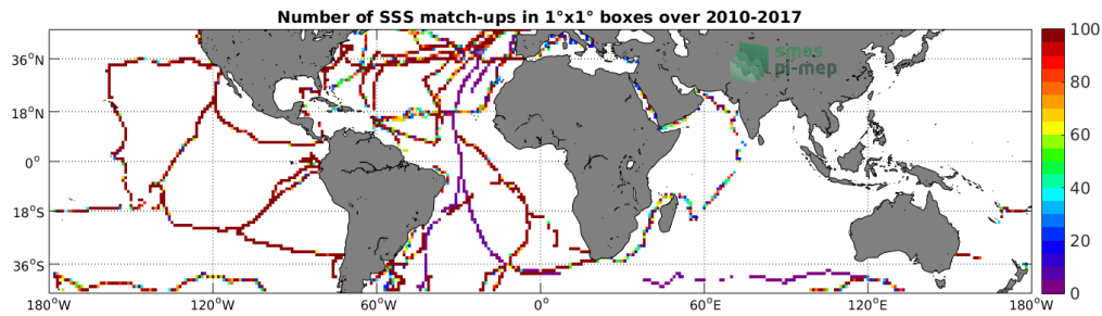
Figure 4: Number of SSS match-ups between TSG (GOSUD-Sailing-ship) SSS and the CCI SSS L4 Merged-OI v2.31 - 7-day running (ESA) SSS product for the Mid-Low Latitudes 45N-45S Pi-MEP region over 1^\circ \times 1^\circ boxes and for the full satellite product period.
