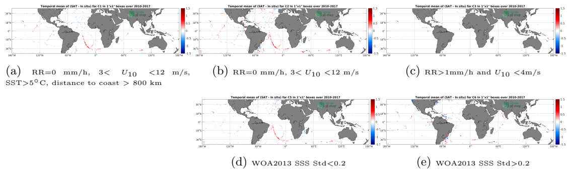
Figure 12: Temporal mean gridded over spatial boxes of size 1^\circ \times 1^\circ of \Delta SSS (CCI SSS L4 Merged-OI v2.31 - 7-day running (ESA) - TSG (GOSUD-Sailing-ship)) for 5 different subdatasets corresponding to: RR=0 mm/h, 3 < U_{10} < 12 m/s, SST > 5°C, distance to coast > 800 km (a), RR=0 mm/h, 3 < U_{10} < 12 m/s (b), RR > 1mm/h and U_{10} < 4 m/s (c), WOA2013 SSS Std < 0.2 (d), WOA2013 SSS Std > 0.2 (e).
