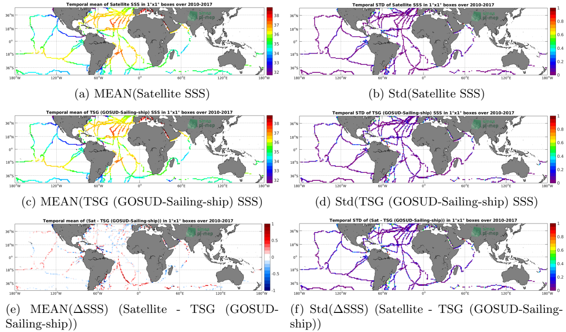
Figure 6: Temporal mean (left) and Std (right) of SSS from CCI SSS L4 Merged-OI v2.31 - 7-day running (ESA) (top), TSG (GOSUD-Sailing-ship) (middle), and of \Delta SSS (Satellite - TSG (GOSUD-Sailing-ship)). Only match-up pairs are used to generate these maps.
