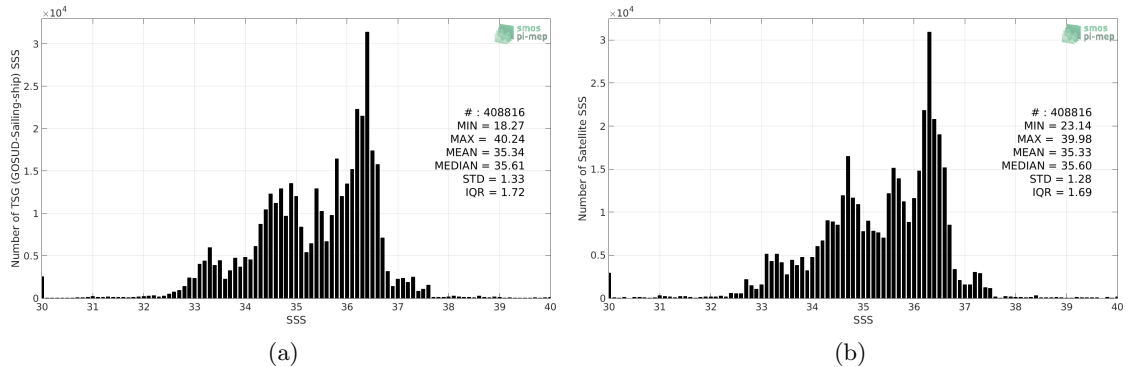
Figure 2: Histograms of SSS from TSG (GOSUD-Sailing-ship) (a) and CCI SSS L4 Merged-OI v2.31 - 7-day running (ESA) (b) considering all match-up pairs per bins of 0.1 over the Mid-Low Latitudes 45N-45S Pi-MEP region and for the full satellite product period.
