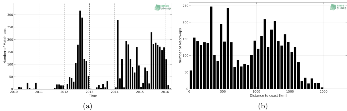
Figure 1: Number of match-ups between Sea mammals and CCI SSS L4 Merged-OI v2.31 - 7-day running (ESA) SSS as a function of time (a) and as function of the distance to coast (b) over the Mid-Low Latitudes 45N-45S Pi-MEP region and for the full satellite product period.
