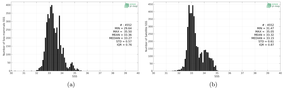
Figure 2: Histograms of SSS from Sea mammals (a) and CCI SSS L4 Merged-OI v2.31 - 7-day running (ESA) (b) considering all match-up pairs per bins of 0.1 over the Mid-Low Latitudes 45N-45S Pi-MEP region and for the full satellite product period.
