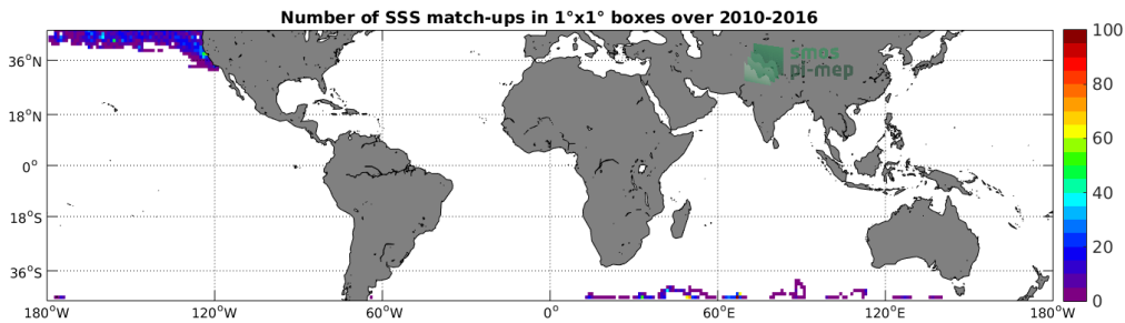
Figure 4: Number of SSS match-ups between Sea mammals SSS and the CCI SSS L4 Merged-OI v2.31 - 7-day running (ESA) SSS product for the Mid-Low Latitudes 45N-45S Pi-MEP region over 1°x1° boxes and for the full satellite product period.
