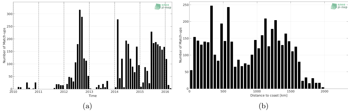
Figure 1: Number of match-ups between Sea mammals and CCI L4 Merged-OI v2.31 - 7-day running (ESA) SSS as a function of time (a) and as function of the distance to coast (b) over the Mid-Low Latitudes 45N-45S Pi-MEP region and for the full satellite product period.
