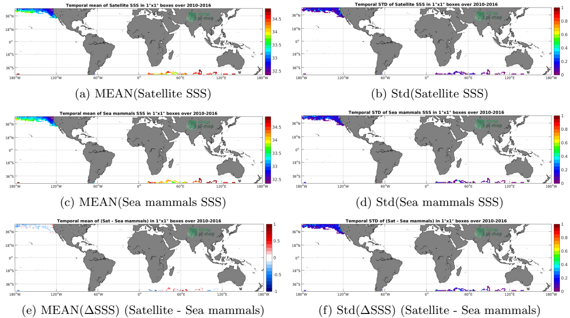
Figure 6: Temporal mean (left) and Std (right) of SSS from CCI L4 Merged-OI v2.31 - 7-day running (ESA) (top), Sea mammals (middle), and of \Delta SSS (Satellite - Sea mammals). Only match-up pairs are used to generate these maps.
