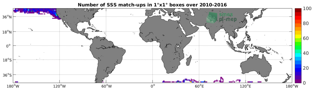
Figure 4: Number of SSS match-ups between Sea mammals SSS and the CCI L4 Merged-OI v2.31 - 7-day running (ESA) SSS product for the Mid-Low Latitudes 45N-45S Pi-MEP region over 1°x1° boxes and for the full satellite product period.
