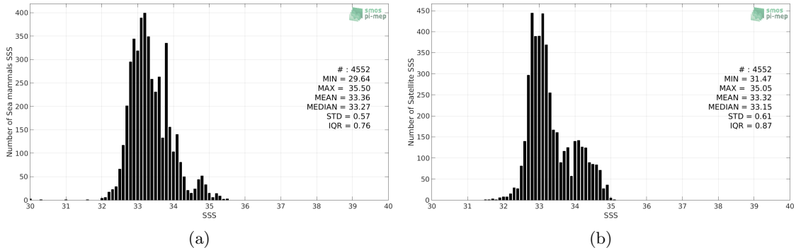
Figure 2: Histograms of SSS from Sea mammals (a) and CCI L4 Merged-OI v2.31 - 7-day running (ESA) (b) considering all match-up pairs per bins of 0.1 over the Mid-Low Latitudes 45N-45S Pi-MEP region and for the full satellite product period.
