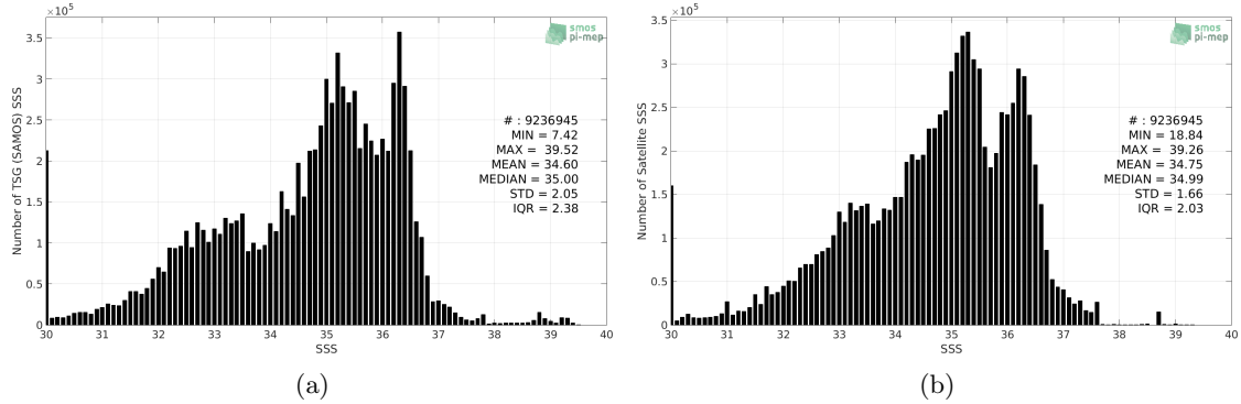
Figure 2: Histograms of SSS from TSG (SAMOS) (a) and CCI SSS L4 Merged-OI v2.31 - 30-day running (ESA) (b) considering all match-up pairs per bins of 0.1 over the Mid-Low Latitudes 45N-45S Pi-MEP region and for the full satellite product period.
