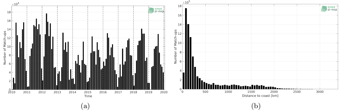
Figure 1: Number of match-ups between TSG (SAMOS) and CCI SSS L4 Merged-OI v2.31 - 30-day running (ESA) SSS as a function of time (a) and as function of the distance to coast (b) over the Mid-Low Latitudes 45N-45S Pi-MEP region and for the full satellite product period.
