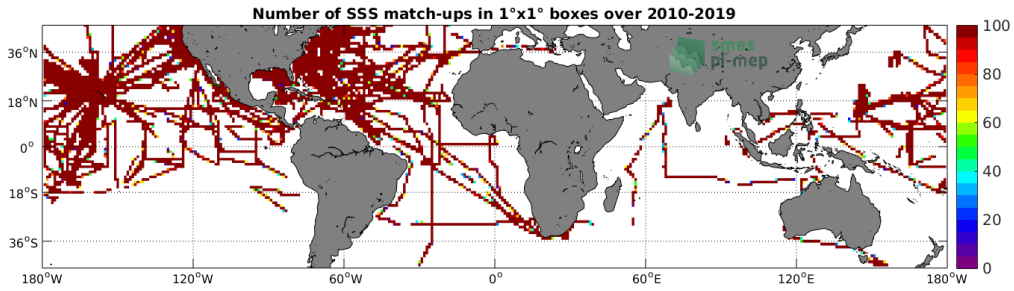
Figure 4: Number of SSS match-ups between TSG (SAMOS) SSS and the CCI L4 Merged-OI v2.31 - 30-day running (ESA) SSS product for the Mid-Low Latitudes 45N-45S Pi-MEP region over 1°x1° boxes and for the full satellite product period.
