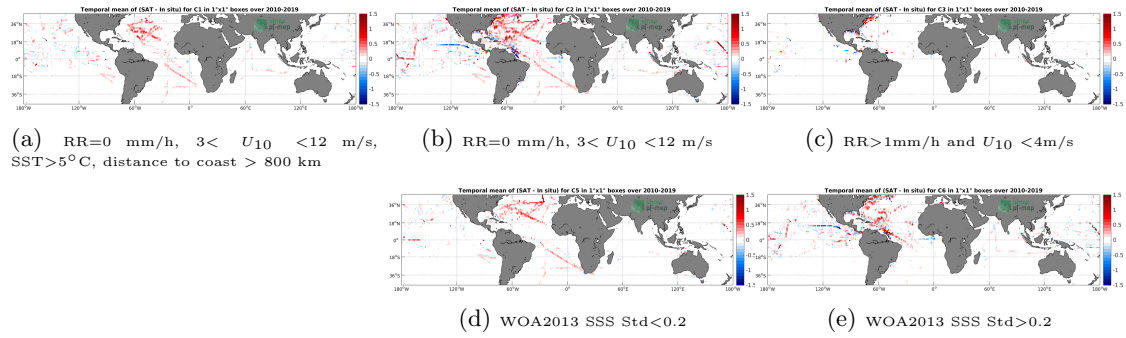
Figure 12: Temporal mean gridded over spatial boxes of size 1^\circ \times 1^\circ of \Delta SSS (CCI L4 Merged-OI v2.31 - 30-day running (ESA) - TSG (SAMOS)) for 5 different subdatasets corresponding to: RR=0 mm/h, 3 < U_{10} < 12 m/s, SST > 5^\circ C , distance to coast > 800 km (a), RR=0 mm/h, 3 < U_{10} < 12 m/s (b), RR > 1 mm/h and U_{10} < 4 m/s (c), WOA2013 SSS Std < 0.2 (d), WOA2013 SSS Std > 0.2 (e).
