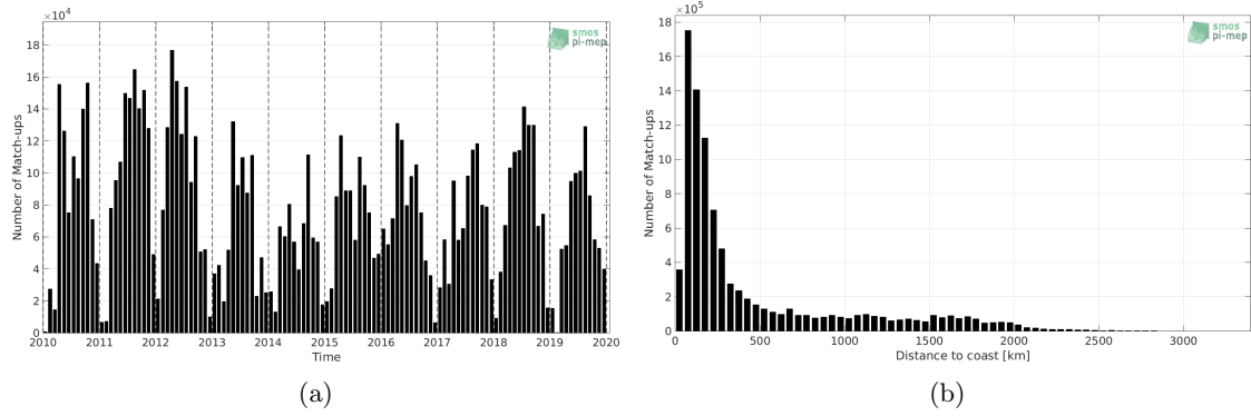
Figure 1: Number of match-ups between TSG (SAMOS) and CCI L4 Merged-OI v2.31 - 30-day running (ESA) SSS as a function of time (a) and as function of the distance to coast (b) over the Mid-Low Latitudes 45N-45S Pi-MEP region and for the full satellite product period.
