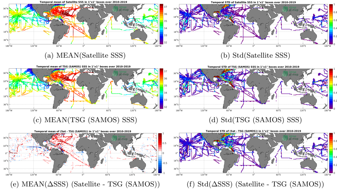
Figure 6: Temporal mean (left) and Std (right) of SSS from CCI L4 Merged-OI v2.31 - 30-day running (ESA) (top), TSG (SAMOS) (middle), and of \Delta SSS (Satellite - TSG (SAMOS)). Only match-up pairs are used to generate these maps.
