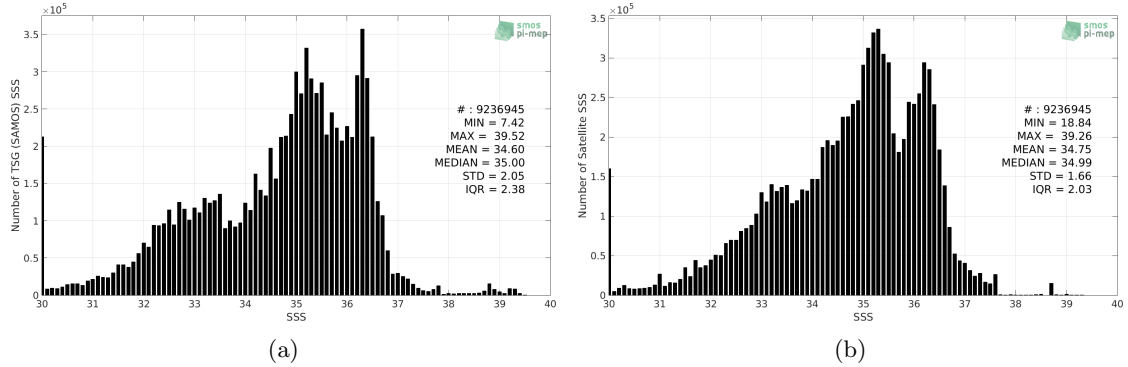
Figure 2: Histograms of SSS from TSG (SAMOS) (a) and CCI L4 Merged-OI v2.31 - 30-day running (ESA) (b) considering all match-up pairs per bins of 0.1 over the Mid-Low Latitudes 45N-45S Pi-MEP region and for the full satellite product period.
