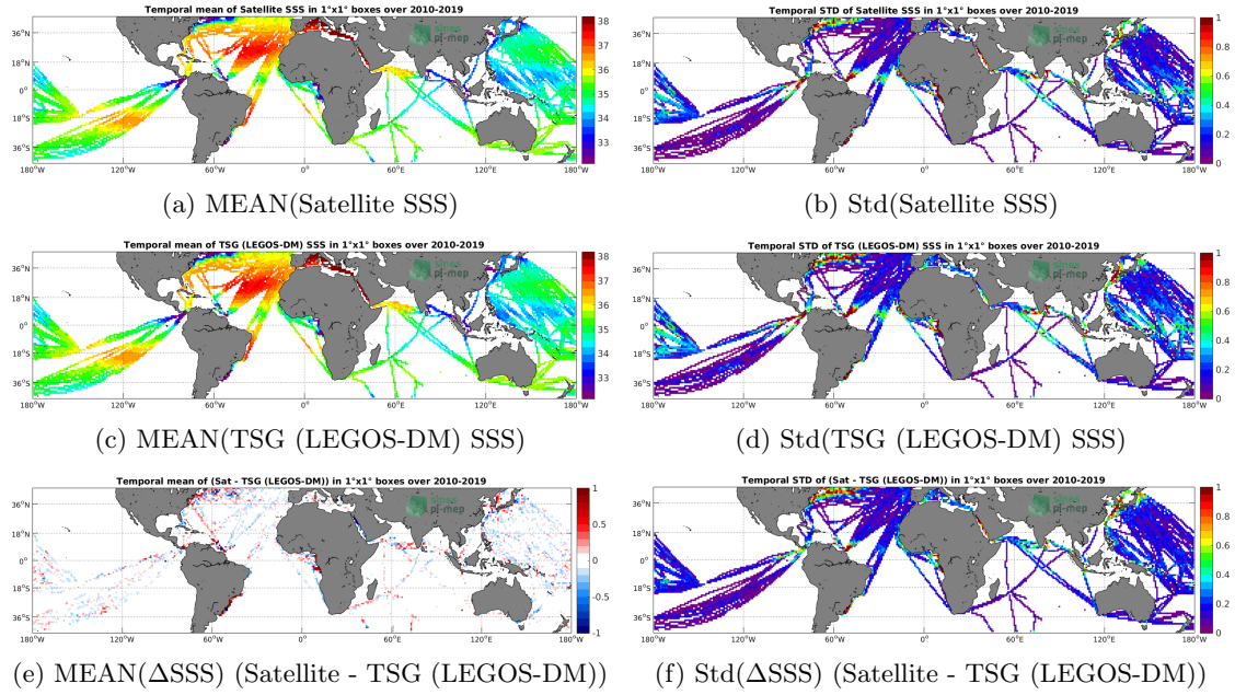
Figure 6: Temporal mean (left) and Std (right) of SSS from CCI SSS L4 Merged-OI v2.31 - 30-day running (ESA) (top), TSG (LEGOS-DM) (middle), and of \Delta SSS (Satellite - TSG (LEGOS-DM)). Only match-up pairs are used to generate these maps.
