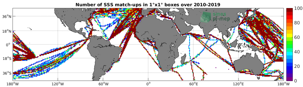
Figure 4: Number of SSS match-ups between TSG (LEGOS-DM) SSS and the CCI SSS L4 Merged-OI v2.31 - 30-day running (ESA) SSS product for the Mid-Low Latitudes 45N-45S Pi-MEP region over 1°x1° boxes and for the full satellite product period.
