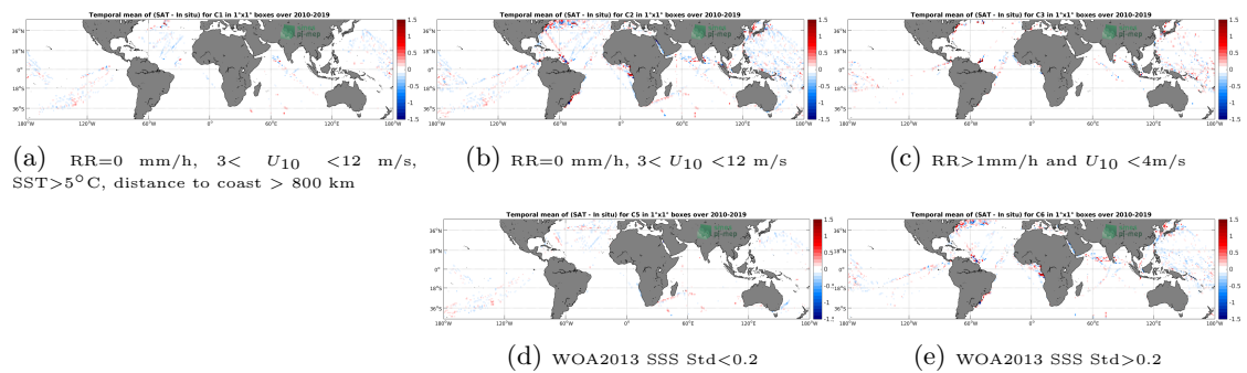
Figure 12: Temporal mean gridded over spatial boxes of size 1°x1° of \Delta SSS (CCI L4 Merged-OI v2.31 - 30-day running (ESA) - TSG (LEGOS-DM)) for 5 different subdatasets corresponding to:RR=0 mm/h, 3 < U_{10} < 12 m/s, SST>5°C, distance to coast > 800 km (a), RR=0 mm/h, 3 < U_{10} < 12 m/s (b), RR>1mm/h and U_{10} < 4 m/s (c), WOA2013 SSS Std<0.2 (d), WOA2013 SSS Std>0.2 (e).
