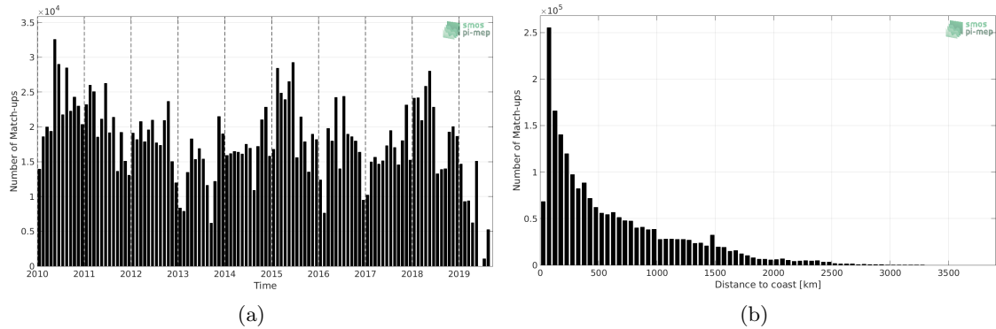
Figure 1: Number of match-ups between TSG (LEGOS-DM) and CCI L4 Merged-OI v2.31 - 30-day running (ESA) SSS as a function of time (a) and as function of the distance to coast (b) over the Mid-Low Latitudes 45N-45S Pi-MEP region and for the full satellite product period.
