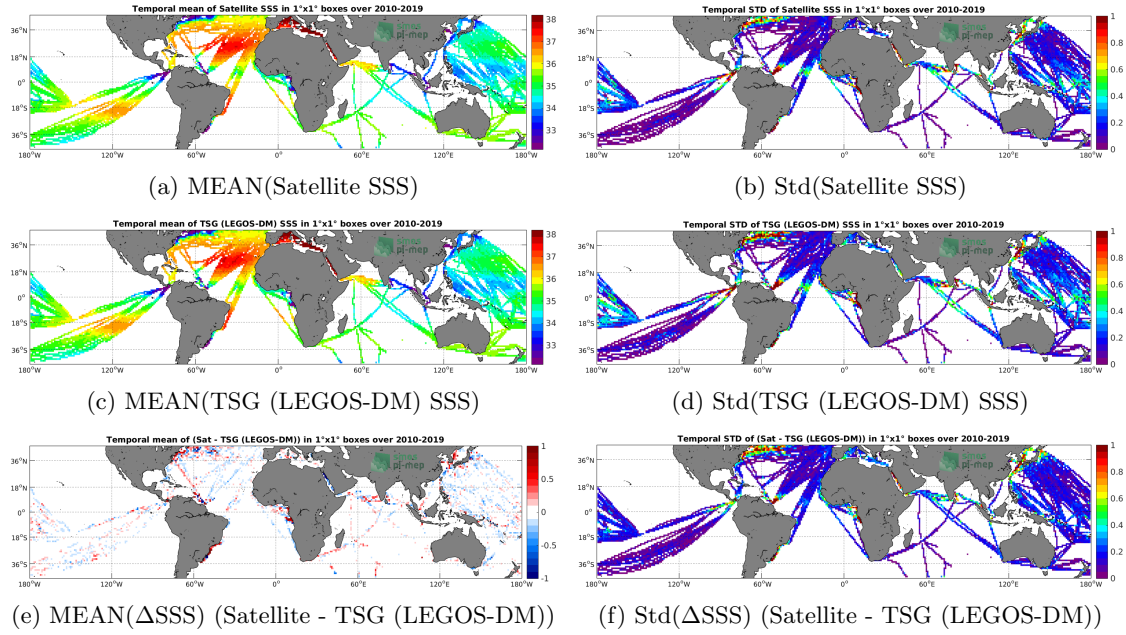
Figure 6: Temporal mean (left) and Std (right) of SSS from CCI L4 Merged-OI v2.31 - 30-day running (ESA) (top), TSG (LEGOS-DM) (middle), and of \Delta SSS (Satellite - TSG (LEGOS-DM)). Only match-up pairs are used to generate these maps.
