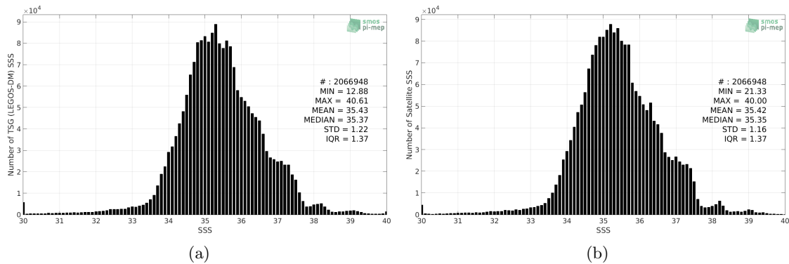
Figure 2: Histograms of SSS from TSG (LEGOS-DM) (a) and CCI L4 Merged-OI v2.31 - 30-day running (ESA) (b) considering all match-up pairs per bins of 0.1 over the Mid-Low Latitudes 45N-45S Pi-MEP region and for the full satellite product period.
