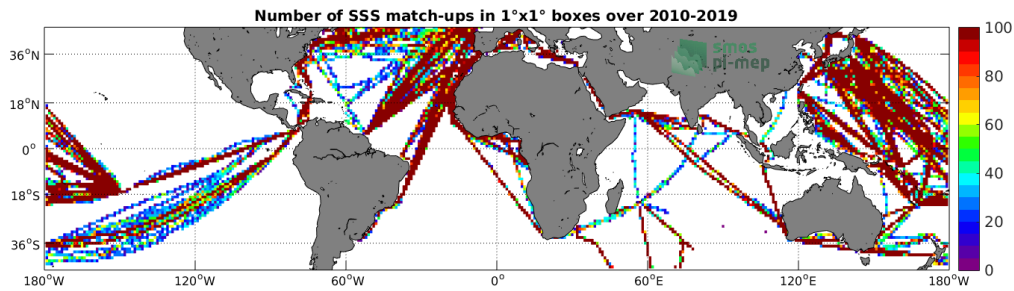
Figure 4: Number of SSS match-ups between TSG (LEGOS-DM) SSS and the CCI L4 Merged-OI v2.31 - 30-day running (ESA) SSS product for the Mid-Low Latitudes 45N-45S Pi-MEP region over 1°x1° boxes and for the full satellite product period.
