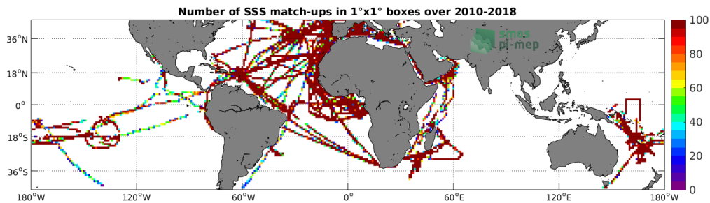
Figure 4: Number of SSS match-ups between TSG (GOSUD-Research-vessel) SSS and the CCI SSS L4 Merged-OI v2.31 - 30-day running (ESA) SSS product for the Mid-Low Latitudes 45N-45S Pi-MEP region over 1°x1° boxes and for the full satellite product period.
