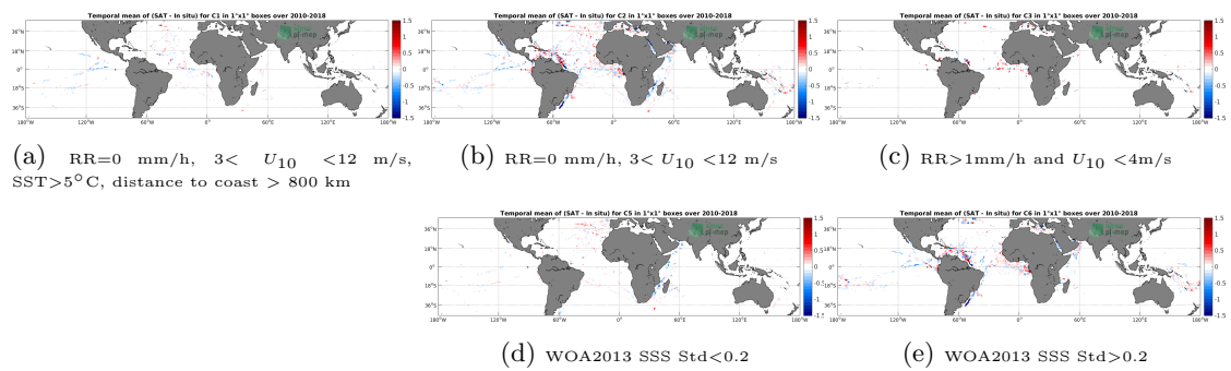
Figure 12: Temporal mean gridded over spatial boxes of size 1^\circ \times 1^\circ of \Delta\text{SSS} (CCI SSS L4 Merged-OI v2.31 - 30-day running (ESA) - TSG (GOSUD-Research-vessel)) for 5 different subdatasets corresponding to:RR=0 mm/h, 3 < U_{10} < 12 m/s, SST>5°C, distance to coast > 800 km (a), RR=0 mm/h, 3 < U_{10} < 12 m/s (b), RR>1mm/h and U_{10} < 4 m/s (c), WOA2013 SSS Std<0.2 (d), WOA2013 SSS Std>0.2 (e).
