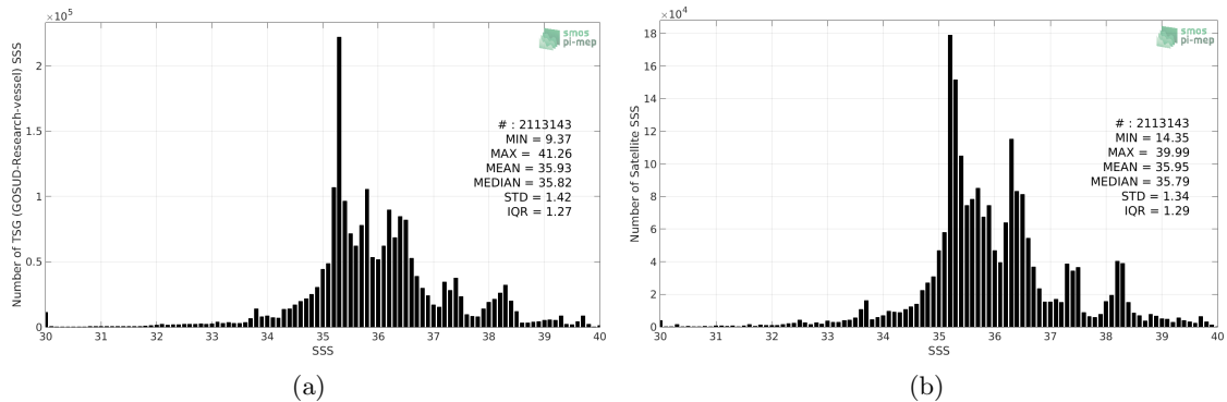
Figure 2: Histograms of SSS from TSG (GOSUD-Research-vessel) (a) and CCI SSS L4 Merged-OI v2.31 - 30-day running (ESA) (b) considering all match-up pairs per bins of 0.1 over the Mid-Low Latitudes 45N-45S Pi-MEP region and for the full satellite product period.
