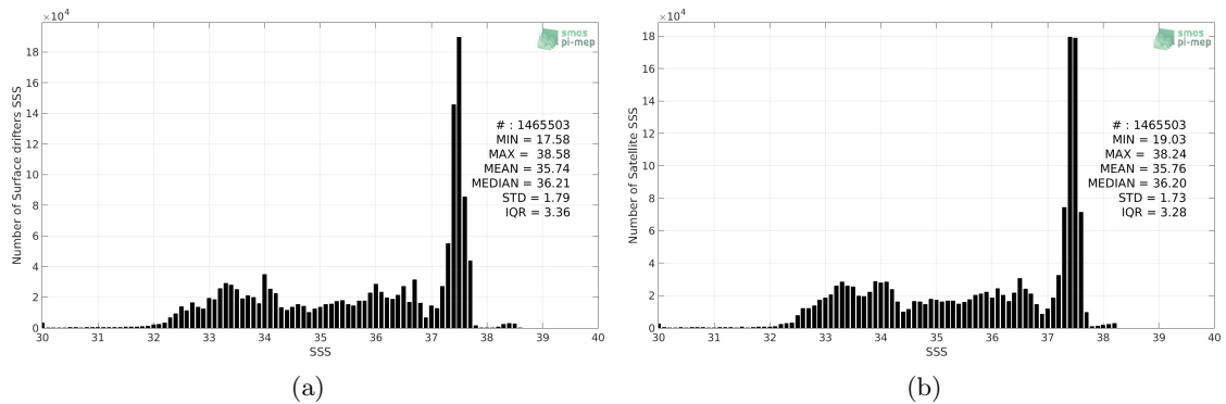
Figure 2: Histograms of SSS from Surface drifters (a) and CCI SSS L4 Merged-OI v2.31 - 30-day running (ESA) (b) considering all match-up pairs per bins of 0.1 over the Mid-Low Latitudes 45N-45S Pi-MEP region and for the full satellite product period.
