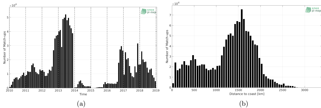
Figure 1: Number of match-ups between Surface drifters and CCI SSS L4 Merged-OI v2.31 - 30-day running (ESA) SSS as a function of time (a) and as function of the distance to coast (b) over the Mid-Low Latitudes 45N-45S Pi-MEP region and for the full satellite product period.
