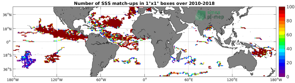
Figure 3: Number of SSS match-ups between Surface drifters SSS and the CCI SSS L4 Merged-OI v2.31 - 30-day running (ESA) SSS product for the Mid-Low Latitudes 45N-45S Pi-MEP region over 1^\circ \times 1^\circ boxes and for the full satellite product period.
