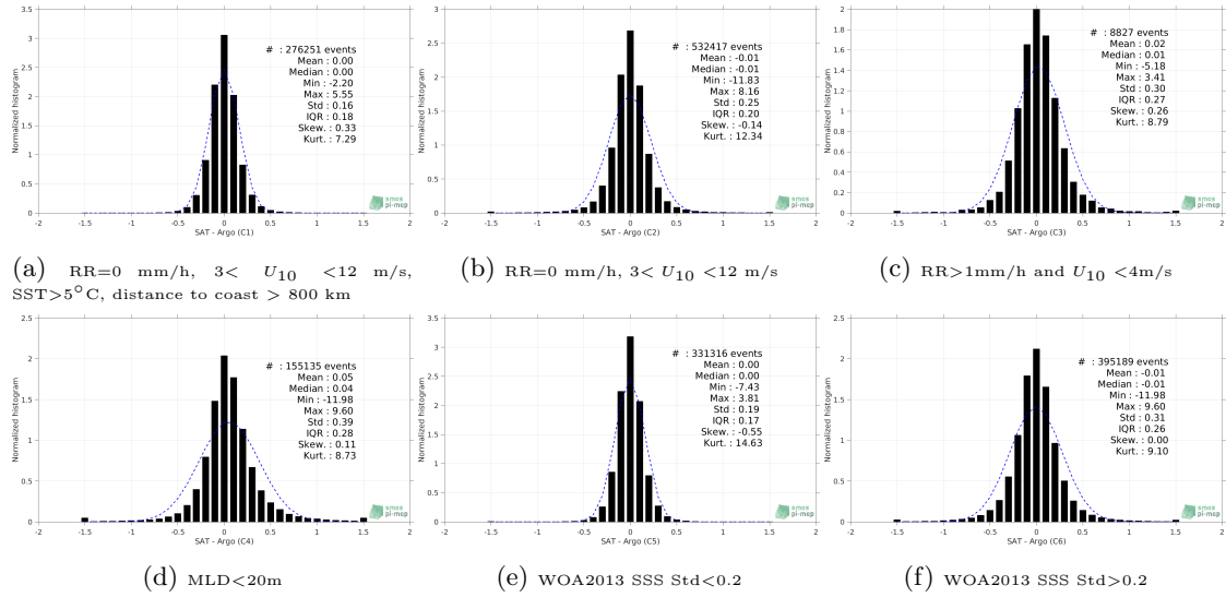
Figure 13: Normalized histograms of \Delta SSS (CCI SSS L4 Merged-OI v2.31 - 30-day running (ESA) - Argo) for 6 different subdatasets corresponding to: RR=0 mm/h, 3 < U_{10} < 12 m/s, SST > 5°C, distance to coast > 800 km (a), RR=0 mm/h, 3 < U_{10} < 12 m/s (b), RR > 1mm/h and U_{10} < 4 m/s (c), MLD < 20m (d), WOA2013 SSS Std < 0.2 (e), WOA2013 SSS Std > 0.2 (f).
