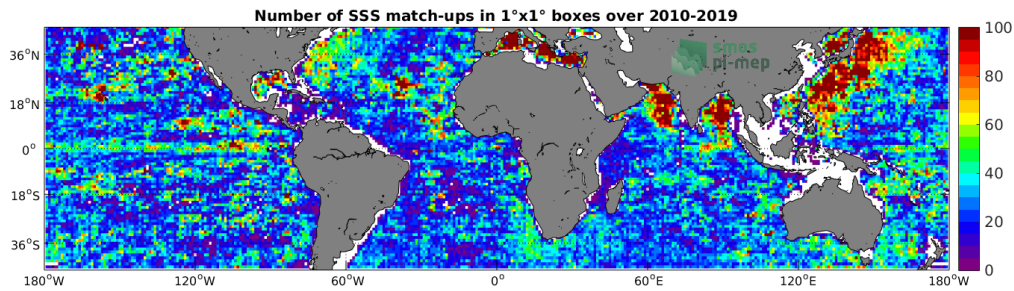
Figure 4: Number of SSS match-ups between Argo SSS and the CCI SSS L4 Merged-OI v2.31 - 30-day running (ESA) SSS product for the Mid-Low Latitudes 45N-45S Pi-MEP region over 1^\circ \times 1^\circ boxes and for the full satellite product period.
