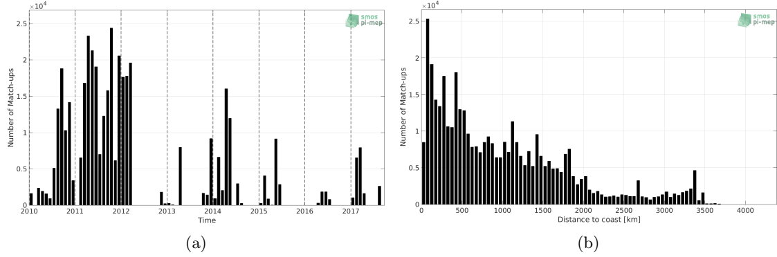
Figure 1: Number of match-ups between TSG-GOSUD-Sailing-ship and CCI L4 Merged-OI v1.8 - 30-day running (ESA) SSS as a function of time (a) and as function of the distance to coast (b) over the Mid-Low Latitudes 45N-45S Pi-MEP region and for the full satellite product period.
