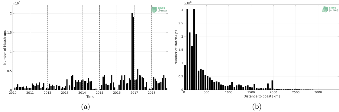
Figure 1: Number of match-ups between TSG-GOSUD-Research-vessel and CCI-L4-ESA-MERGED-OI-V1.8-30DAY-RUNNING SSS as a function of time (a) and as function of the distance to coast (b) over the Mid-Low Latitudes 45N-45S Pi-MEP region and for the full satellite product period.
