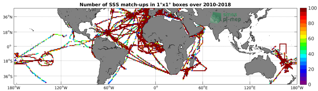
Figure 4: Number of SSS match-ups between TSG-GOSUD-Research-vessel SSS and the CCI-L4-ESA-MERGED-OI-V1.8-30DAY-RUNNING SSS product for the Mid-Low Latitudes 45N-45S Pi-MEP region over 1^\circ \times 1^\circ boxes and for the full satellite product period.
