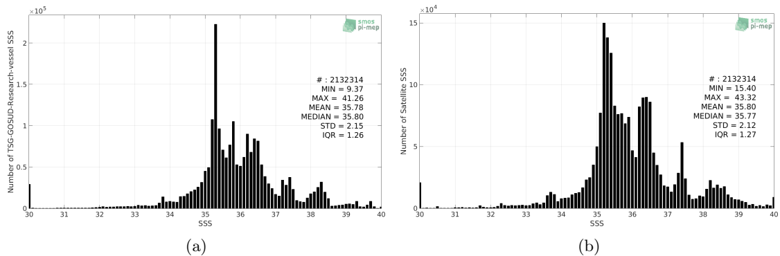
Figure 2: Histograms of SSS from TSG-GOSUD-Research-vessel (a) and CCI-L4-ESA-MERGED-OI-V1.8-30DAY-RUNNING (b) considering all match-up pairs per bins of 0.1 over the Mid-Low Latitudes 45N-45S Pi-MEP region and for the full satellite product period.
