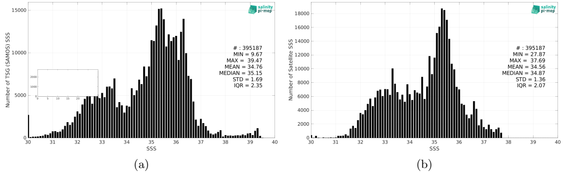
Figure 2: Histograms of SSS from TSG (SAMOS) (a) and Aquarius SSS L4 OI v5 - Weekly (IPRC) (b) considering all match-up pairs per bins of 0.1 over the Mid-Low Latitudes 45N-45S Pi-MEP region and for the full satellite product period.
