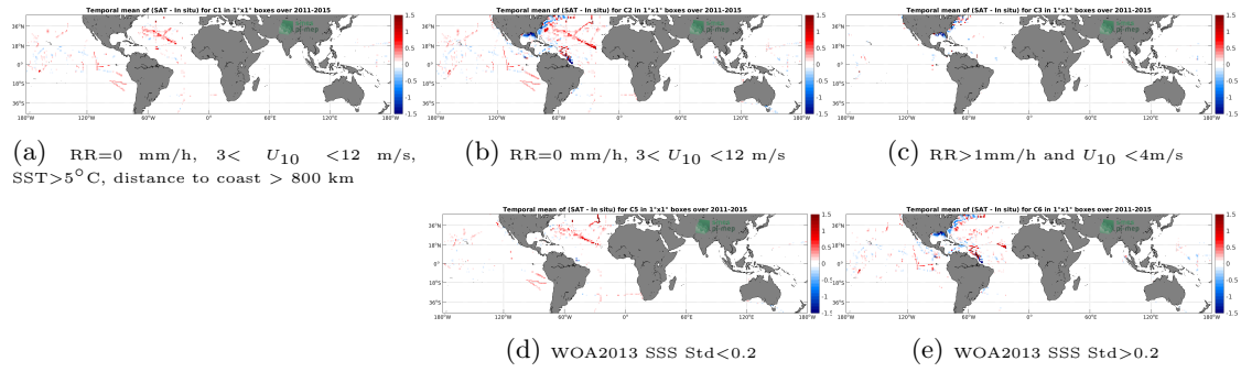
Figure 12: Temporal mean gridded over spatial boxes of size 1^\circ \times 1^\circ of \Delta SSS (Aquarius SSS L4 OI v5 - Weekly (IPRC) - TSG (SAMOS)) for 5 different subdatasets corresponding to: RR=0 mm/h, 3 < U_{10} < 12 m/s, SST > 5^\circ\text{C} , distance to coast > 800 km (a), RR=0 mm/h, 3 < U_{10} < 12 m/s (b), RR > 1 mm/h and U_{10} < 4 m/s (c), WOA2013 SSS Std < 0.2 (d), WOA2013 SSS Std > 0.2 (e).
