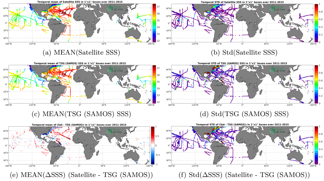
Figure 6: Temporal mean (left) and Std (right) of SSS from Aquarius SSS L4 OI v5 - Weekly (IPRC) (top), TSG (SAMOS) (middle), and of \Delta SSS (Satellite - TSG (SAMOS)). Only match-up pairs are used to generate these maps.
