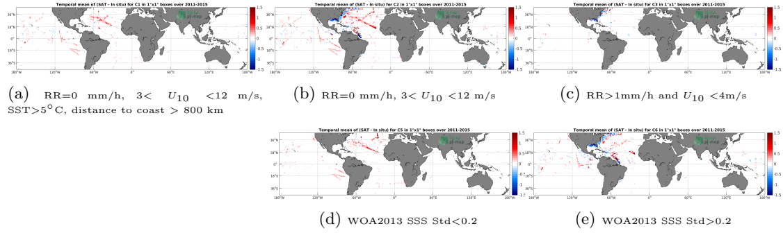
Figure 12: Temporal mean gridded over spatial boxes of size 1^\circ \times 1^\circ of \Delta SSS (Aquarius-L4-IPRC-V5-WEEKLY - TSG-SAMOS) for 5 different subdatasets corresponding to: RR=0 mm/h, 3 < U_{10} < 12 m/s, SST >5^\circ\text{C} , distance to coast > 800 km (a), RR=0 mm/h, 3 < U_{10} < 12 m/s (b), RR >1 mm/h and U_{10} < 4 m/s (c), WOA2013 SSS Std <0.2 (d), WOA2013 SSS Std >0.2 (e).
