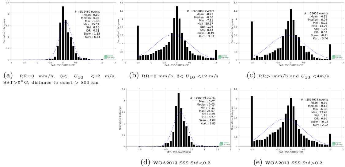
Figure 13: Normalized histogram of \Delta SSS (Aquarius-L4-IPRC-V5-WEEKLY - TSG-SAMOS) for 5 different subdatasets corresponding to: RR=0 mm/h, 3 < U_{10} < 12 m/s, SST >5^\circ\text{C} , distance to coast > 800 km (a), RR=0 mm/h, 3 < U_{10} < 12 m/s (b), RR >1 mm/h and U_{10} < 4 m/s (c), WOA2013 SSS Std <0.2 (d), WOA2013 SSS Std >0.2 (e).
