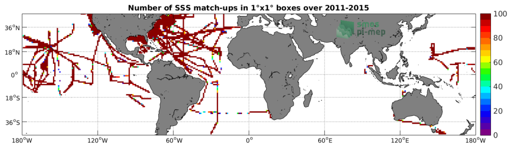
Figure 4: Number of SSS match-ups between TSG-SAMOS SSS and the Aquarius-L4-IPRC-V5-WEEKLY SSS product for the Mid-Low Latitudes 45N-45S Pi-MEP region over 1^\circ \times 1^\circ boxes and for the full satellite product period.
