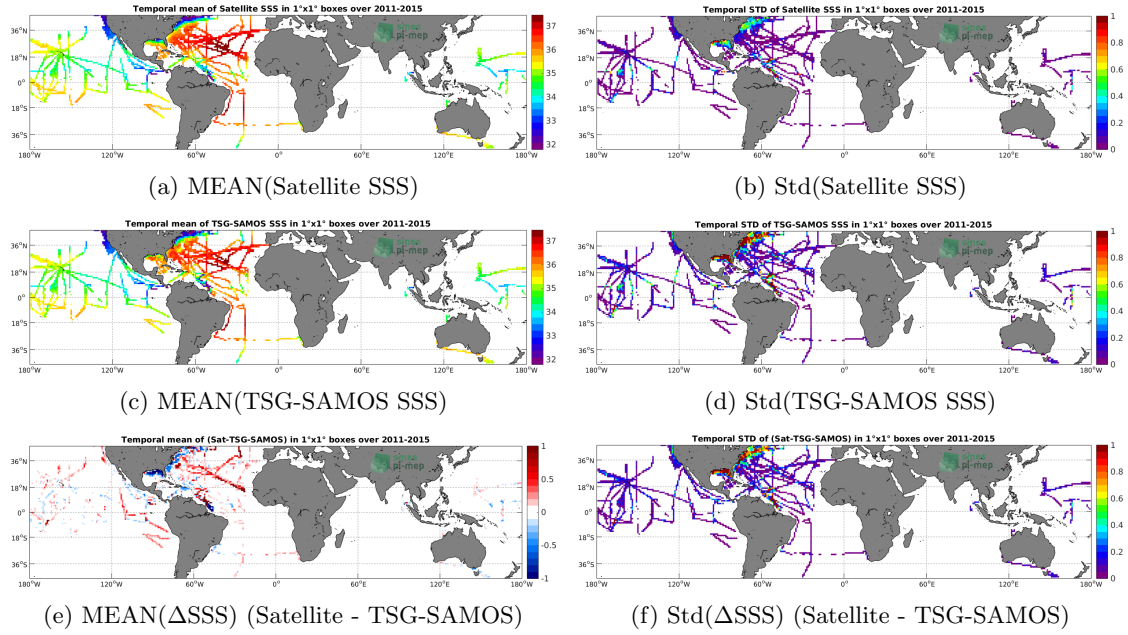
Figure 6: Temporal mean (left) and Std (right) of SSS from Aquarius-L4-IPRC-V5-WEEKLY (top), TSG-SAMOS (middle), and of \Delta SSS (Satellite - TSG-SAMOS). Only match-up pairs are used to generate these maps.
