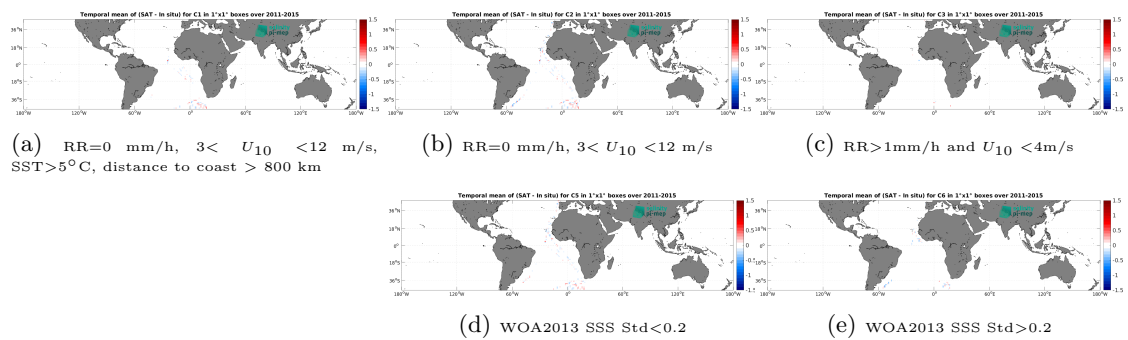
Figure 14: Temporal mean gridded over spatial boxes of size 1^\circ \times 1^\circ of \Delta SSS (Aquarius SSS L4 OI v5 - Weekly (IPRC) - TSG (Polarstern)) for 5 different subdatasets corresponding to: RR=0 mm/h, 3 < U_{10} < 12 m/s, SST > 5^\circ\text{C} , distance to coast > 800 km (a), RR=0 mm/h, 3 < U_{10} < 12 m/s (b), RR > 1 mm/h and U_{10} < 4 m/s (c), WOA2013 SSS Std < 0.2 (d), WOA2013 SSS Std > 0.2 (e).
