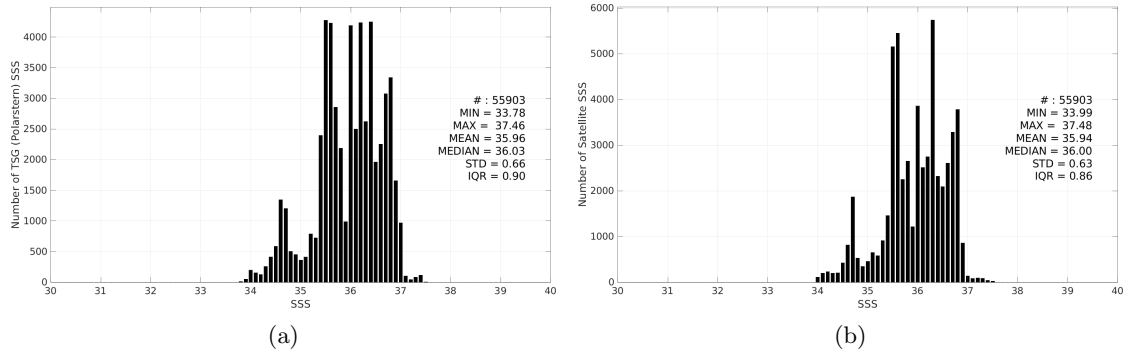
Figure 3: Histograms of SSS from TSG (Polarstern) (a) and Aquarius SSS L4 OI v5 - Weekly (IPRC) (b) considering all match-up pairs per bins of 0.1 over the Mid-Low Latitudes 45N-45S Pi-MEP region and for the full satellite product period.
