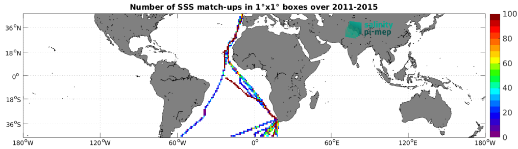
Figure 5: Number of SSS match-ups between TSG (Polarstern) SSS and the Aquarius SSS L4 OI v5 - Weekly (IPRC) SSS product for the Mid-Low Latitudes 45N-45S Pi-MEP region over 1^\circ \times 1^\circ boxes and for the full satellite product period.
