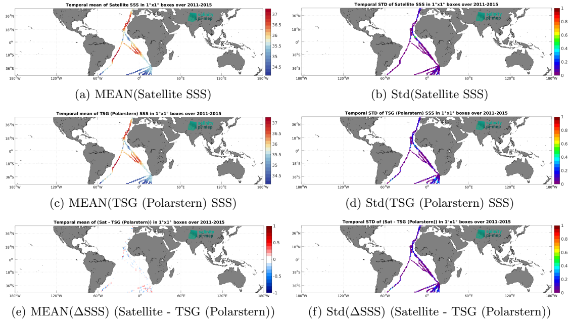
Figure 7: Temporal mean (left) and Std (right) of SSS from Aquarius SSS L4 OI v5 - Weekly (IPRC) (top), TSG (Polarstern) (middle), and of \Delta SSS (Satellite - TSG (Polarstern)). Only match-up pairs are used to generate these maps.
