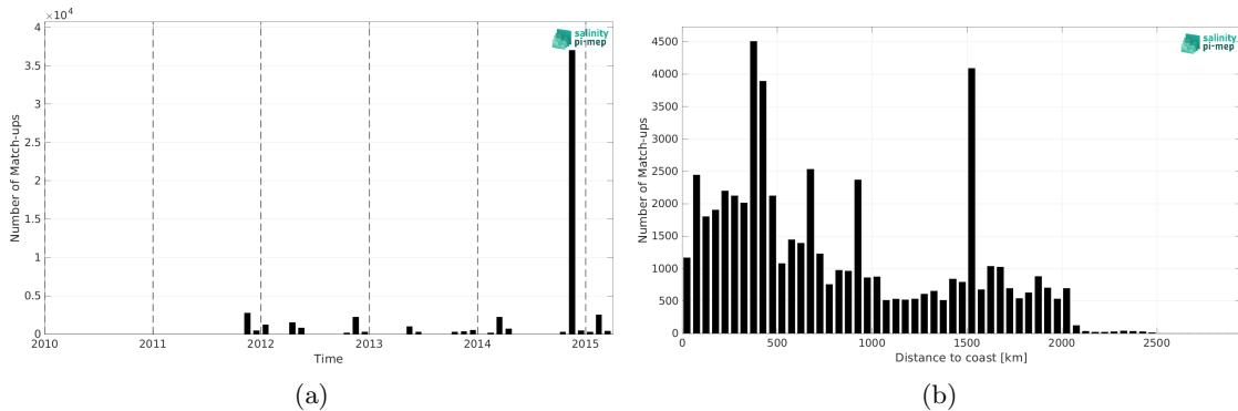
Figure 2: Number of match-ups between TSG (Polarstern) and Aquarius SSS L4 OI v5 - Weekly (IPRC) SSS as a function of time (a) and as function of the distance to coast (b) over the Mid-Low Latitudes 45N-45S Pi-MEP region and for the full satellite product period.
