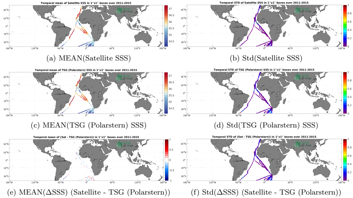
Figure 6: Temporal mean (left) and Std (right) of SSS from Aquarius SSS L4 OI v5 - Weekly (IPRC) (top), TSG (Polarstern) (middle), and of \Delta SSS (Satellite - TSG (Polarstern)). Only match-up pairs are used to generate these maps.
