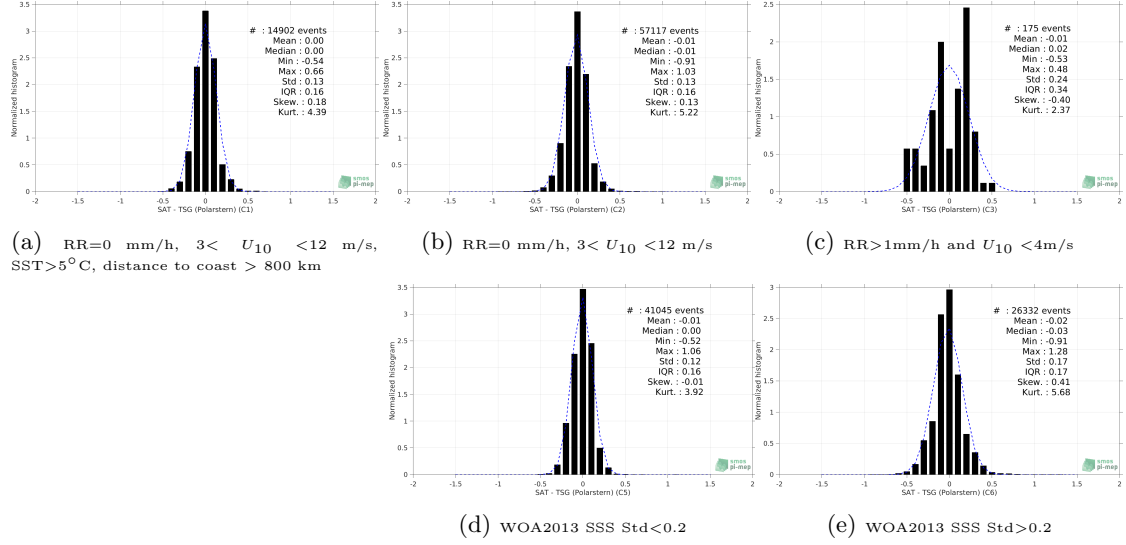
Figure 13: Normalized histogram of \Delta SSS (Aquarius SSS L4 OI v5 - Weekly (IPRC) - TSG (Polarstern)) for 5 different subdatasets corresponding to: RR=0 mm/h, 3 < U_{10} < 12 m/s, SST>5°C, distance to coast > 800 km (a), RR=0 mm/h, 3 < U_{10} < 12 m/s (b), RR>1mm/h and U_{10} < 4 m/s (c), WOA2013 SSS Std<0.2 (d), WOA2013 SSS Std>0.2 (e).
