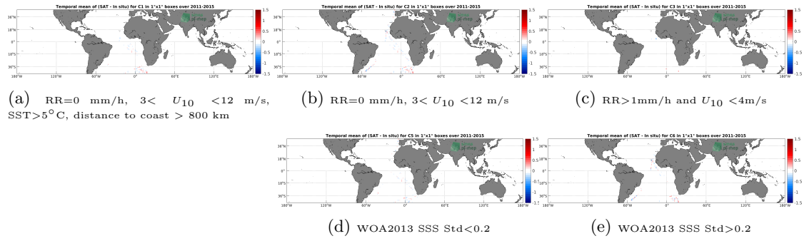
Figure 12: Temporal mean gridded over spatial boxes of size 1^\circ \times 1^\circ of \Delta SSS (Aquarius SSS L4 OI v5 - Weekly (IPRC) - TSG (Polarstern)) for 5 different subdatasets corresponding to: RR=0 mm/h, 3 < U_{10} < 12 m/s, SST > 5^\circ\text{C} , distance to coast > 800 km (a), RR=0 mm/h, 3 < U_{10} < 12 m/s (b), RR > 1 mm/h and U_{10} < 4 m/s (c), WOA2013 SSS Std < 0.2 (d), WOA2013 SSS Std > 0.2 (e).
