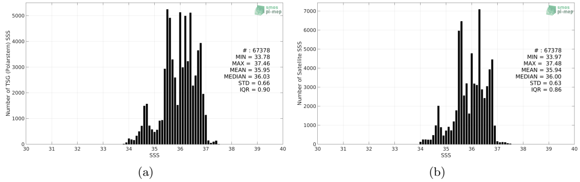
Figure 2: Histograms of SSS from TSG (Polarstern) (a) and Aquarius SSS L4 OI v5 - Weekly (IPRC) (b) considering all match-up pairs per bins of 0.1 over the Mid-Low Latitudes 45N-45S Pi-MEP region and for the full satellite product period.
