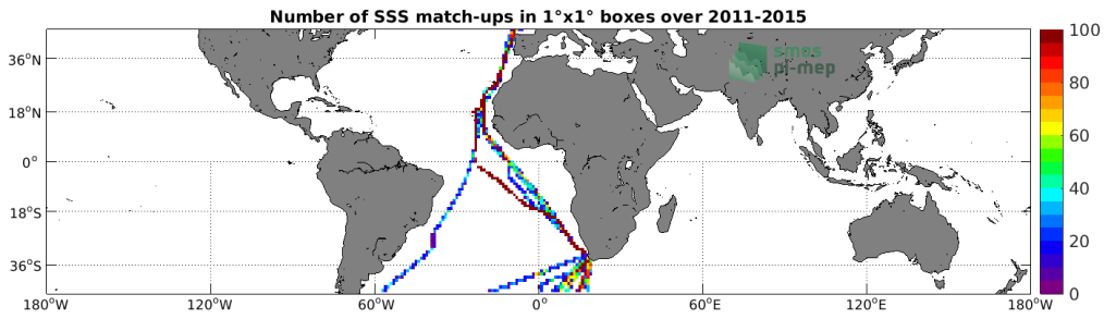
Figure 4: Number of SSS match-ups between TSG (Polarstern) SSS and the Aquarius SSS L4 OI v5 - Weekly (IPRC) SSS product for the Mid-Low Latitudes 45N-45S Pi-MEP region over 1^\circ \times 1^\circ boxes and for the full satellite product period.
