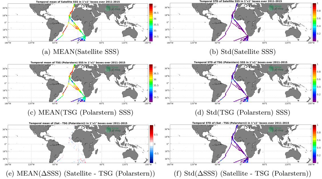
Figure 6: Temporal mean (left) and Std (right) of SSS from Aquarius SSS L4 OI v5 - Weekly (IPRC) (top), TSG (Polarstern) (middle), and of \Delta SSS (Satellite - TSG (Polarstern)). Only match-up pairs are used to generate these maps.
