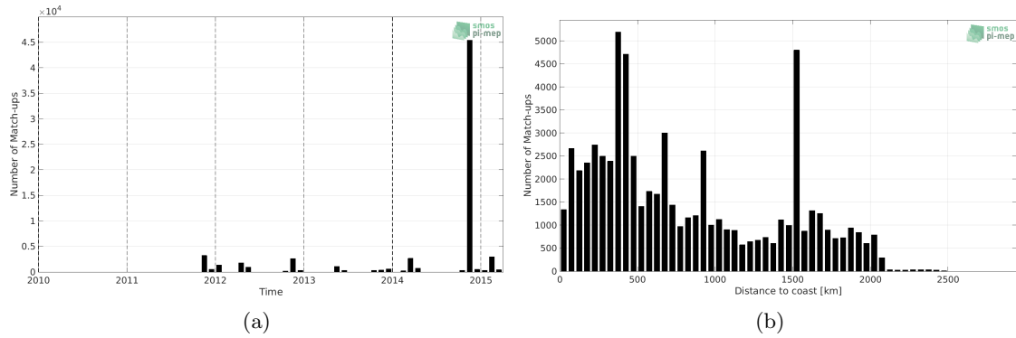
Figure 1: Number of match-ups between TSG (Polarstern) and Aquarius SSS L4 OI v5 - Weekly (IPRC) SSS as a function of time (a) and as function of the distance to coast (b) over the Mid-Low Latitudes 45N-45S Pi-MEP region and for the full satellite product period.
