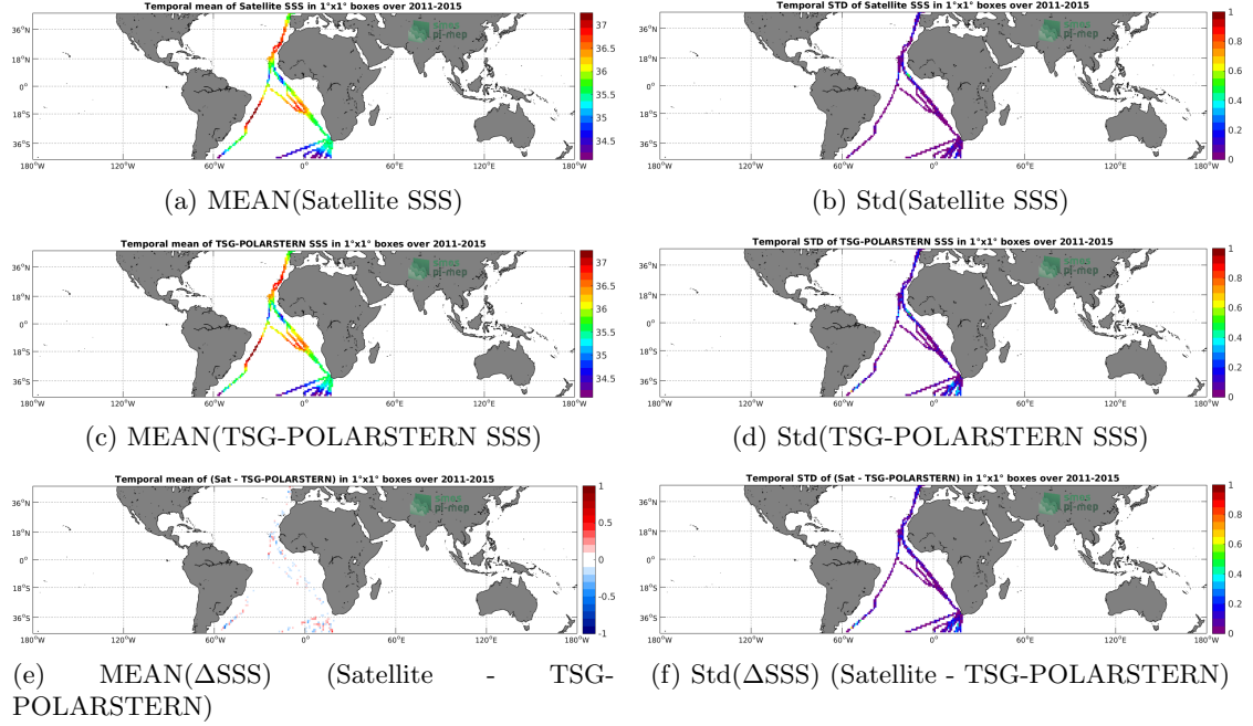
Figure 6: Temporal mean (left) and Std (right) of SSS from Aquarius-L4-IPRC-V5-WEEKLY (top), TSG-POLARSTERN (middle), and of \Delta SSS (Satellite - TSG-POLARSTERN). Only match-up pairs are used to generate these maps.
