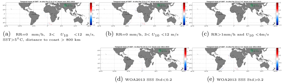
Figure 12: Temporal mean gridded over spatial boxes of size 1^\circ \times 1^\circ of \Delta SSS (Aquarius-L4-IPRC-V5-WEEKLY - TSG-POLARSTERN) for 5 different subdatasets corresponding to: RR=0 mm/h, 3 < U_{10} < 12 m/s, SST > 5^\circ C , distance to coast > 800 km (a), RR=0 mm/h, 3 < U_{10} < 12 m/s (b), RR > 1 mm/h and U_{10} < 4 m/s (c), WOA2013 SSS Std < 0.2 (d), WOA2013 SSS Std > 0.2 (e).
