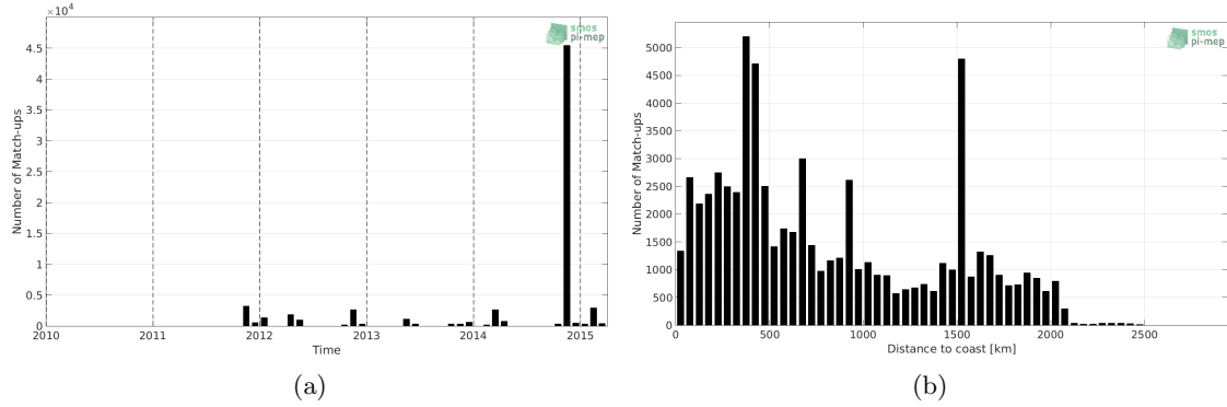
Figure 1: Number of match-ups between TSG-POLARSTERN and Aquarius-L4-IPRC-V5-WEEKLY SSS as a function of time (a) and as function of the distance to coast (b) over the Mid-Low Latitudes 45N-45S Pi-MEP region and for the full satellite product period.
