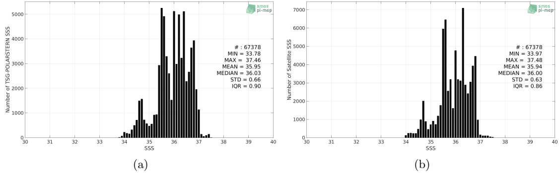
Figure 2: Histograms of SSS from TSG-POLARSTERN (a) and Aquarius-L4-IPRC-V5-WEEKLY (b) considering all match-up pairs per bins of 0.1 over the Mid-Low Latitudes 45N-45S Pi-MEP region and for the full satellite product period.
