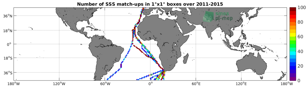
Figure 4: Number of SSS match-ups between TSG-POLARSTERN SSS and the Aquarius-L4-IPRC-V5-WEEKLY SSS product for the Mid-Low Latitudes 45N-45S Pi-MEP region over 1^\circ \times 1^\circ boxes and for the full satellite product period.
