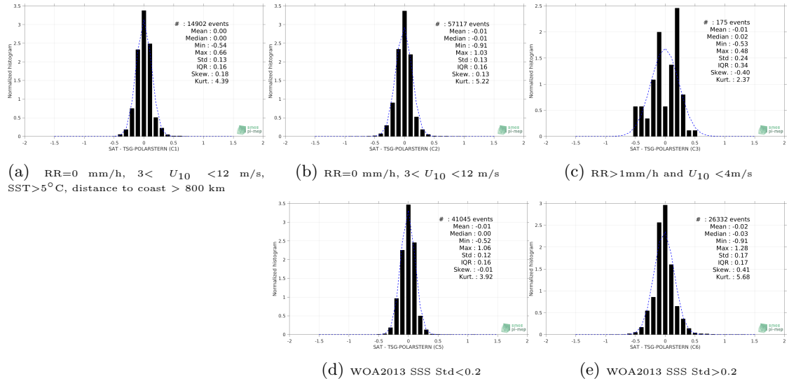
Figure 13: Normalized histogram of \Delta SSS (Aquarius-L4-IPRC-V5-WEEKLY - TSG-POLARSTERN) for 5 different subdatasets corresponding to: RR=0 mm/h, 3 < U_{10} < 12 m/s, SST > 5^\circ C , distance to coast > 800 km (a), RR=0 mm/h, 3 < U_{10} < 12 m/s (b), RR > 1 mm/h and U_{10} < 4 m/s (c), WOA2013 SSS Std < 0.2 (d), WOA2013 SSS Std > 0.2 (e).
