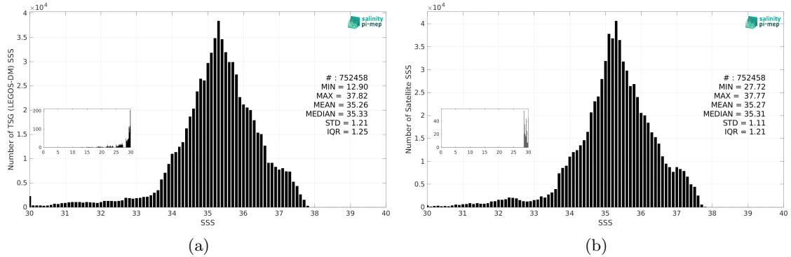
Figure 3: Histograms of SSS from TSG (LEGOS-DM) (a) and Aquarius SSS L4 OI v5 - Weekly (IPRC) (b) considering all match-up pairs per bins of 0.1 over the Mid-Low Latitudes 45N-45S Pi-MEP region and for the full satellite product period.
