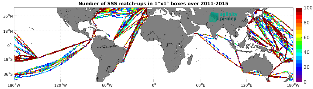
Figure 5: Number of SSS match-ups between TSG (LEGOS-DM) SSS and the Aquarius SSS L4 OI v5 - Weekly (IPRC) SSS product for the Mid-Low Latitudes 45N-45S Pi-MEP region over 1^\circ \times 1^\circ boxes and for the full satellite product period.
