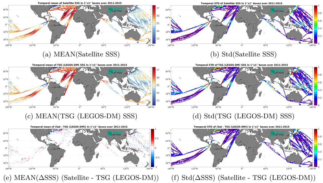
Figure 7: Temporal mean (left) and Std (right) of SSS from Aquarius SSS L4 OI v5 - Weekly (IPRC) (top), TSG (LEGOS-DM) (middle), and of \Delta SSS (Satellite - TSG (LEGOS-DM)). Only match-up pairs are used to generate these maps.
