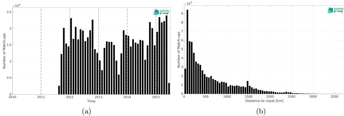
Figure 2: Number of match-ups between TSG (LEGOS-DM) and Aquarius SSS L4 OI v5 - Weekly (IPRC) SSS as a function of time (a) and as function of the distance to coast (b) over the Mid-Low Latitudes 45N-45S Pi-MEP region and for the full satellite product period.
