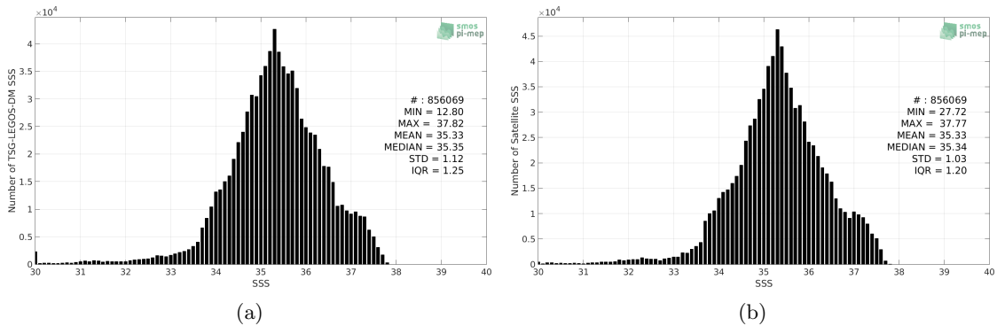
Figure 2: Histograms of SSS from TSG-LEGOS-DM (a) and Aquarius-L4-IPRC-V5-WEEKLY (b) considering all match-up pairs per bins of 0.1 over the Mid-Low Latitudes 45N-45S Pi-MEP region and for the full satellite product period.
