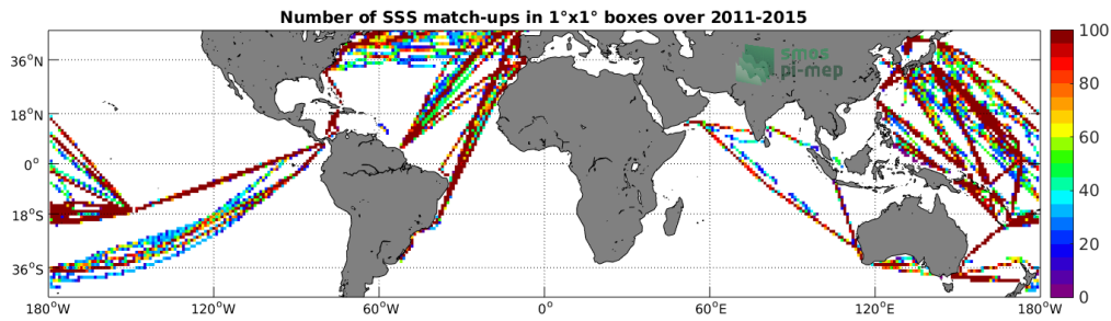
Figure 4: Number of SSS match-ups between TSG-LEGOS-DM SSS and the Aquarius-L4-IPRC-V5-WEEKLY SSS product for the Mid-Low Latitudes 45N-45S Pi-MEP region over 1^\circ \times 1^\circ boxes and for the full satellite product period.
