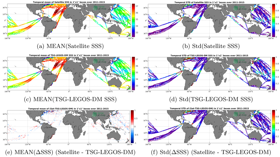
Figure 6: Temporal mean (left) and Std (right) of SSS from Aquarius-L4-IPRC-V5-WEEKLY (top), TSG-LEGOS-DM (middle), and of \Delta SSS (Satellite - TSG-LEGOS-DM). Only match-up pairs are used to generate these maps.
