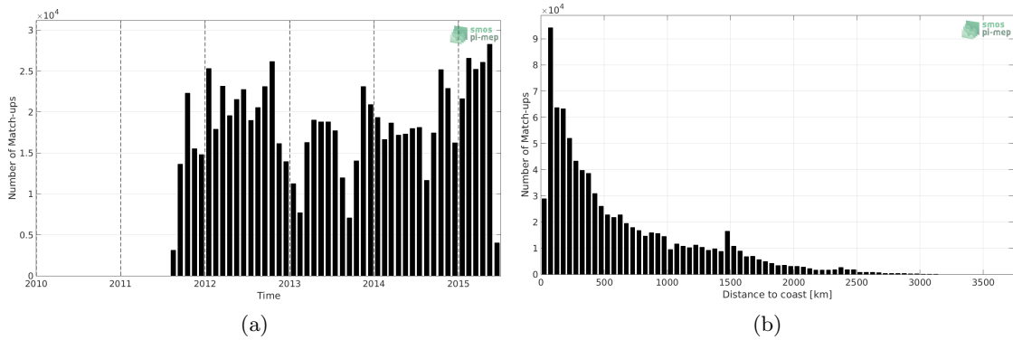
Figure 1: Number of match-ups between TSG-LEGOS-DM and Aquarius-L4-IPRC-V5-WEEKLY SSS as a function of time (a) and as function of the distance to coast (b) over the Mid-Low Latitudes 45N-45S Pi-MEP region and for the full satellite product period.
