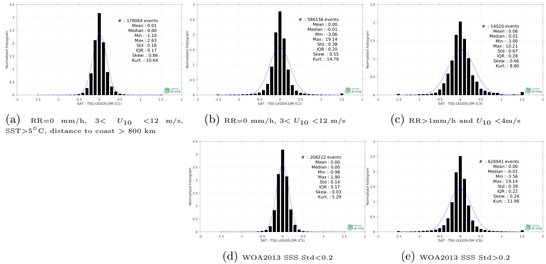
Figure 13: Normalized histogram of \Delta SSS (Aquarius-L4-IPRC-V5-WEEKLY - TSG-LEGOS-DM) for 5 different subdatasets corresponding to: RR=0 mm/h, 3 < U_{10} < 12 m/s, SST >5^\circ\text{C} , distance to coast > 800 km (a), RR=0 mm/h, 3 < U_{10} < 12 m/s (b), RR >1 mm/h and U_{10} < 4 m/s (c), WOA2013 SSS Std <0.2 (d), WOA2013 SSS Std >0.2 (e).
