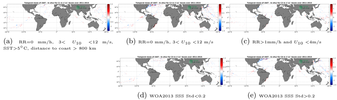
Figure 12: Temporal mean gridded over spatial boxes of size 1^\circ \times 1^\circ of \Delta SSS (Aquarius-L4-IPRC-V5-WEEKLY - TSG-LEGOS-DM) for 5 different subdatasets corresponding to: RR=0 mm/h, 3 < U_{10} < 12 m/s, SST >5^\circ\text{C} , distance to coast > 800 km (a), RR=0 mm/h, 3 < U_{10} < 12 m/s (b), RR >1 mm/h and U_{10} < 4 m/s (c), WOA2013 SSS Std <0.2 (d), WOA2013 SSS Std >0.2 (e).
