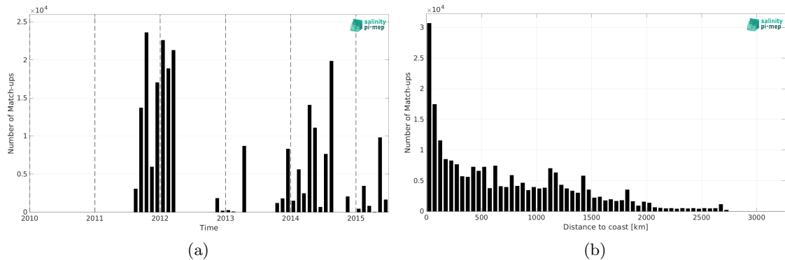
Figure 2: Number of match-ups between TSG (GOSUD-Sailing-ship) and Aquarius SSS L4 OI v5 - Weekly (IPRC) SSS as a function of time (a) and as function of the distance to coast (b) over the Mid-Low Latitudes 45N-45S Pi-MEP region and for the full satellite product period.
