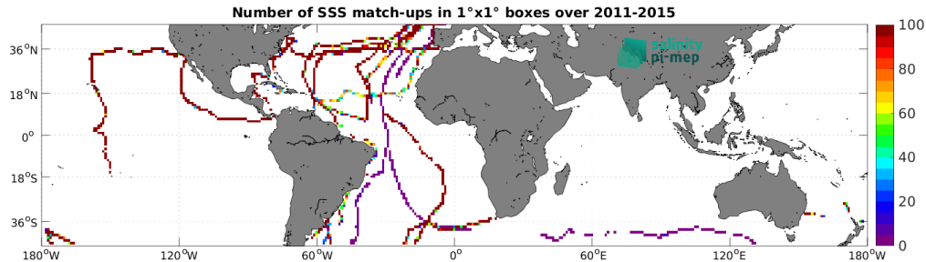
Figure 5: Number of SSS match-ups between TSG (GOSUD-Sailing-ship) SSS and the Aquarius SSS L4 OI v5 - Weekly (IPRC) SSS product for the Mid-Low Latitudes 45N-45S Pi-MEP region over 1^\circ \times 1^\circ boxes and for the full satellite product period.
