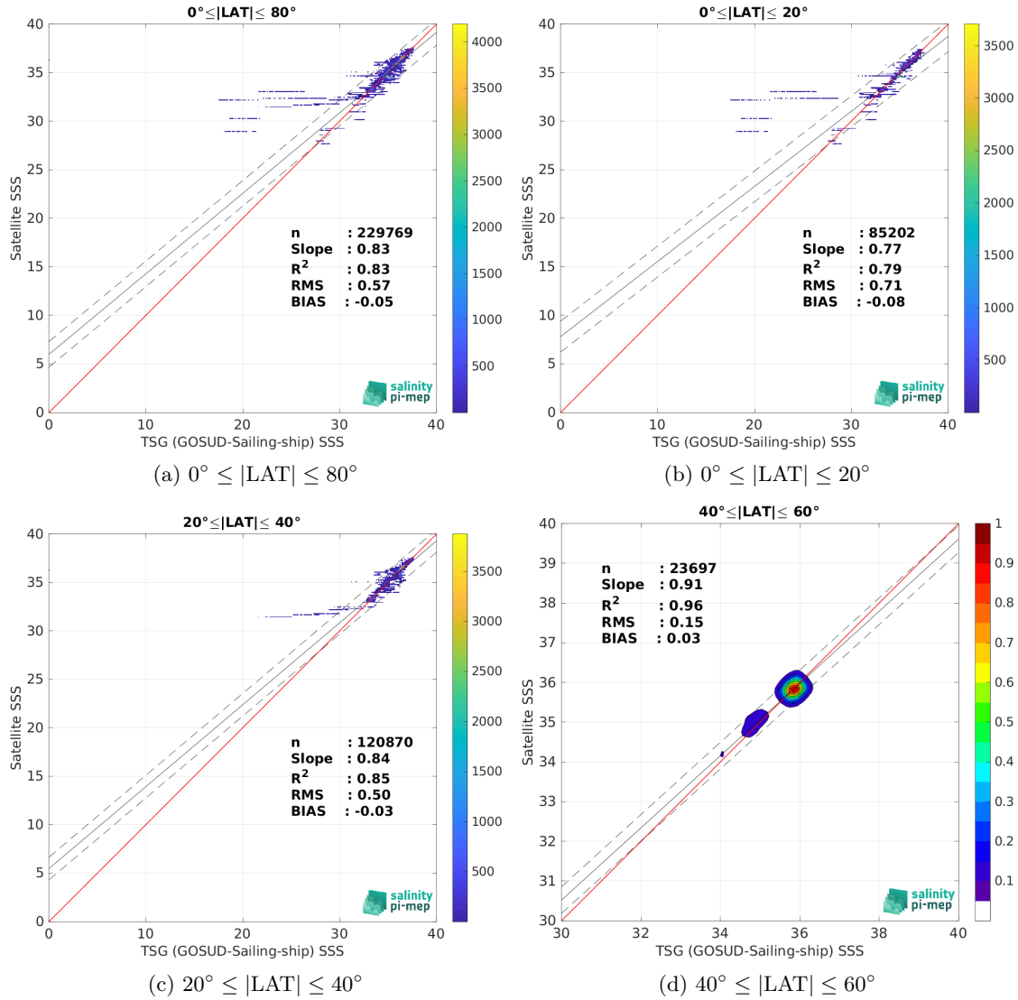
Figure 10: Contour maps of the concentration of Aquarius SSS L4 OI v5 - Weekly (IPRC) SSS (y-axis) versus TSG (GOSUD-Sailing-ship) SSS (x-axis) at match-up pairs for different latitude bands. For each plot, the red line shows x=y . The black thin and dashed lines indicate a linear fit through the data cloud and the \pm 95\% confidence levels, respectively. The number match-up pairs n , the slope and R^2 coefficient of the linear fit, the root mean square (RMS) and the mean bias between satellite and in situ data are indicated for each latitude band in each plots.
