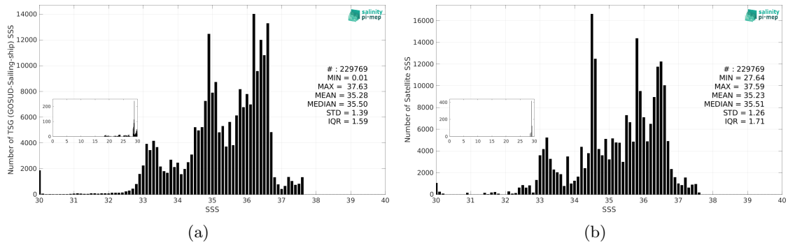
Figure 3: Histograms of SSS from TSG (GOSUD-Sailing-ship) (a) and Aquarius SSS L4 OI v5 - Weekly (IPRC) (b) considering all match-up pairs per bins of 0.1 over the Mid-Low Latitudes 45N-45S Pi-MEP region and for the full satellite product period.
