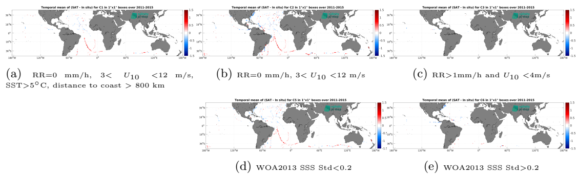
Figure 14: Temporal mean gridded over spatial boxes of size 1^\circ \times 1^\circ of \Delta\text{SSS} (Aquarius SSS L4 OI v5 - Weekly (IPRC) - TSG (GOSUD-Sailing-ship)) for 5 different subdatasets corresponding to:RR=0 mm/h, 3 < U_{10} < 12 m/s, SST>5°C, distance to coast > 800 km (a), RR=0 mm/h, 3 < U_{10} < 12 m/s (b), RR>1mm/h and U_{10} < 4 m/s (c), WOA2013 SSS Std<0.2 (d), WOA2013 SSS Std>0.2 (e).
