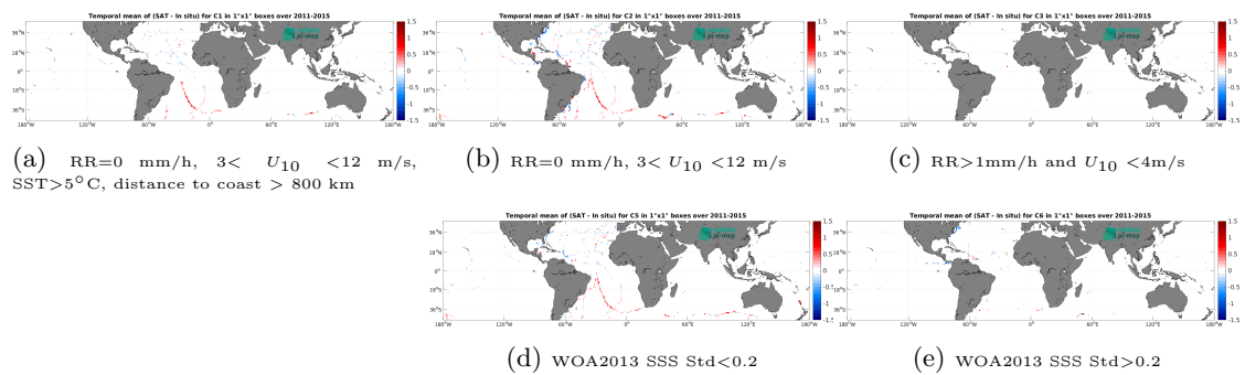
Figure 12: Temporal mean gridded over spatial boxes of size 1^\circ \times 1^\circ of \Delta\text{SSS} (Aquarius SSS L4 OI v5 - Weekly (IPRC) - TSG (GOSUD-Sailing-ship)) for 5 different subdatasets corresponding to:RR=0 mm/h, 3 < U_{10} < 12 m/s, SST>5°C, distance to coast > 800 km (a), RR=0 mm/h, 3 < U_{10} < 12 m/s (b), RR>1mm/h and U_{10} < 4 m/s (c), WOA2013 SSS Std<0.2 (d), WOA2013 SSS Std>0.2 (e).
