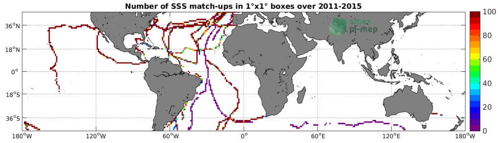
Figure 4: Number of SSS match-ups between TSG-GOSUD-Sailing-ship SSS and the Aquarius-L4-IPRC-V5-WEEKLY SSS product for the Mid-Low Latitudes 45N-45S Pi-MEP region over 1°x1° boxes and for the full satellite product period.
