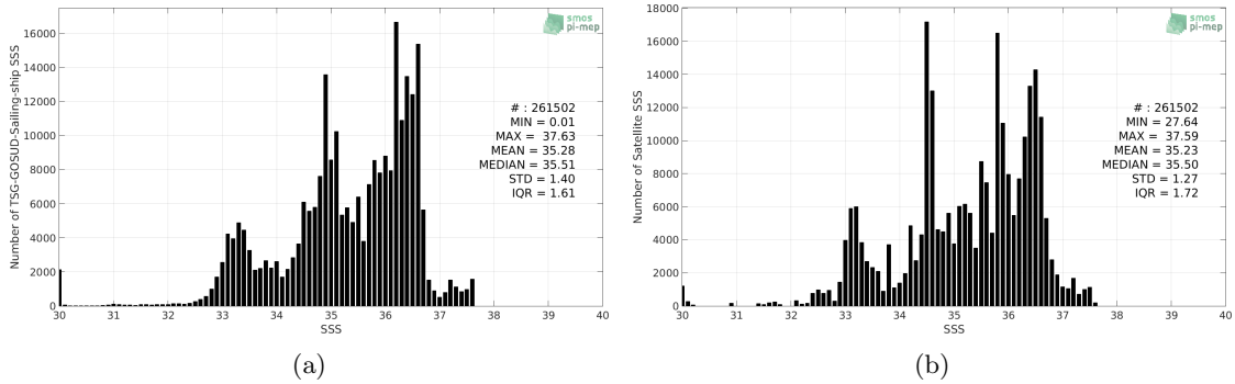
Figure 2: Histograms of SSS from TSG-GOSUD-Sailing-ship (a) and Aquarius-L4-IPRC-V5-WEEKLY (b) considering all match-up pairs per bins of 0.1 over the Mid-Low Latitudes 45N-45S Pi-MEP region and for the full satellite product period.
