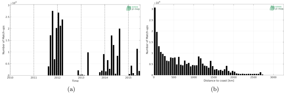
Figure 1: Number of match-ups between TSG-GOSUD-Sailing-ship and Aquarius-L4-IPRC-V5-WEEKLY SSS as a function of time (a) and as function of the distance to coast (b) over the Mid-Low Latitudes 45N-45S Pi-MEP region and for the full satellite product period.
