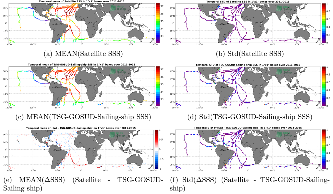
Figure 6: Temporal mean (left) and Std (right) of SSS from Aquarius-L4-IPRC-V5-WEEKLY (top), TSG-GOSUD-Sailing-ship (middle), and of \Delta SSS (Satellite - TSG-GOSUD-Sailing-ship). Only match-up pairs are used to generate these maps.
