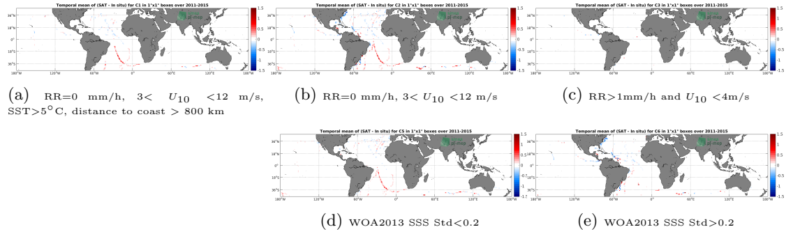
Figure 12: Temporal mean gridded over spatial boxes of size 1^\circ \times 1^\circ of \Delta SSS (Aquarius-L4-IPRC-V5-WEEKLY - TSG-GOSUD-Sailing-ship) for 5 different subdatasets corresponding to: RR=0 mm/h, 3 < U_{10} < 12 m/s, SST > 5^\circ C , distance to coast > 800 km (a), RR=0 mm/h, 3 < U_{10} < 12 m/s (b), RR > 1 mm/h and U_{10} < 4 m/s (c), WOA2013 SSS Std < 0.2 (d), WOA2013 SSS Std > 0.2 (e).
