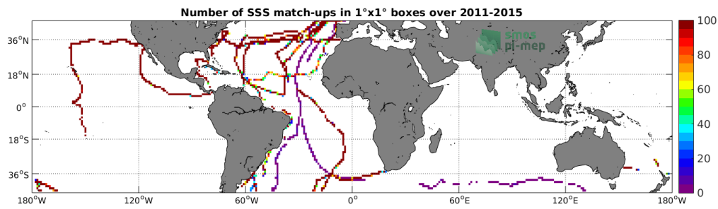
Figure 4: Number of SSS match-ups between TSG-GOSUD-Sailing-ship SSS and the Aquarius-L4-IPRC-V5-WEEKLY SSS product for the Mid-Low Latitudes 45N-45S Pi-MEP region over 1^\circ \times 1^\circ boxes and for the full satellite product period.
