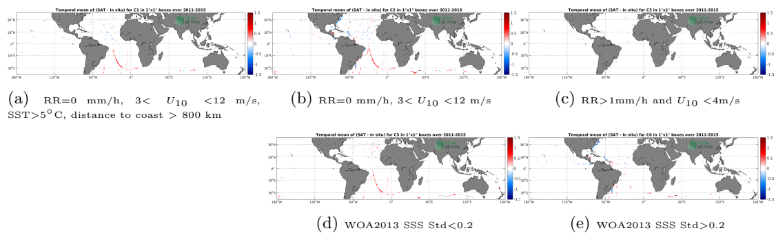
Figure 12: Temporal mean gridded over spatial boxes of size 1^\circ \times 1^\circ of \Delta SSS (Aquarius-L4-IPRC-V5-WEEKLY - TSG-GOSUD-Sailing-ship) for 5 different subdatasets corresponding to:RR=0 mm/h, 3 < U_{10} < 12 m/s, SST >5^\circ\text{C} , distance to coast > 800 km (a), RR=0 mm/h, 3 < U_{10} < 12 m/s (b), RR >1 mm/h and U_{10} < 4 m/s (c), WOA2013 SSS Std <0.2 (d), WOA2013 SSS Std >0.2 (e).
