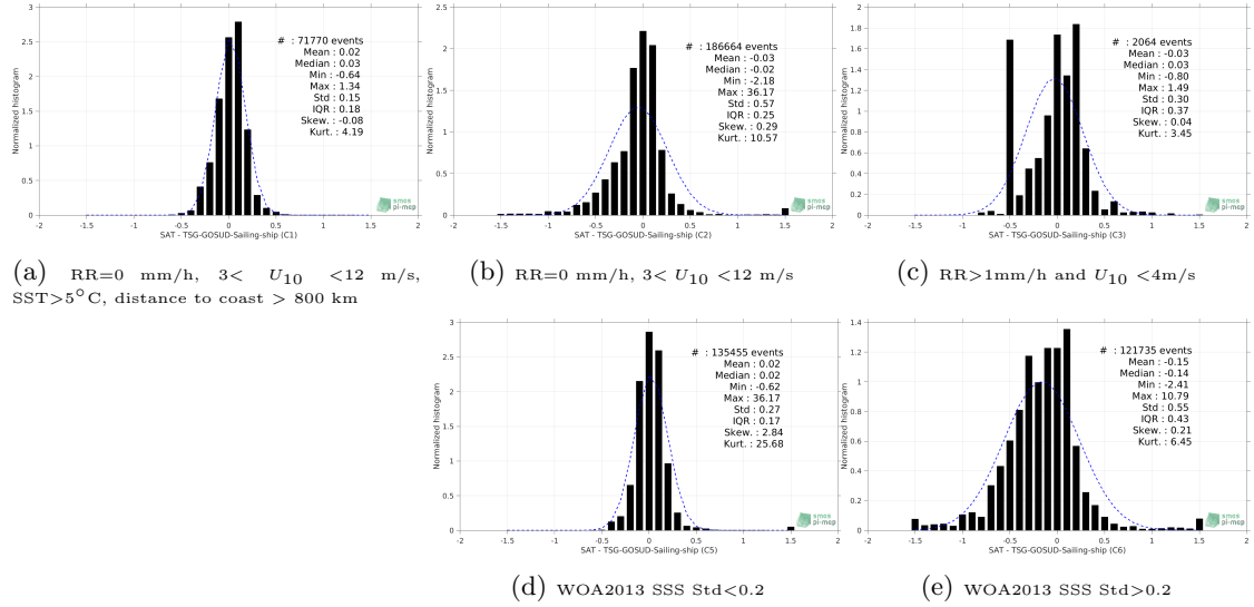
Figure 13: Normalized histogram of \Delta\text{SSS} (Aquarius-L4-IPRC-V5-WEEKLY - TSG-GOSUD-Sailing-ship) for 5 different subdatasets corresponding to: RR=0 mm/h, 3 < U_{10} < 12 m/s, SST>5°C, distance to coast > 800 km (a), RR=0 mm/h, 3 < U_{10} < 12 m/s (b), RR>1mm/h and U_{10} < 4 m/s (c), WOA2013 SSS Std<0.2 (d), WOA2013 SSS Std>0.2 (e).
