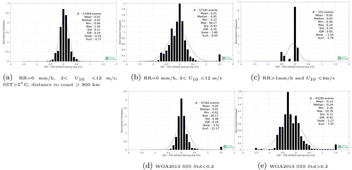
Figure 13: Normalized histogram of \Delta SSS (Aquarius-L4-IPRC-V5-WEEKLY - TSG-GOSUD-Sailing-ship) for 5 different subdatasets corresponding to: RR=0 mm/h, 3 < U_{10} < 12 m/s, SST >5^\circ C, distance to coast > 800 km (a), RR=0 mm/h, 3 < U_{10} < 12 m/s (b), RR >1 mm/h and U_{10} < 4 m/s (c), WOA2013 SSS Std <0.2 (d), WOA2013 SSS Std >0.2 (e).
