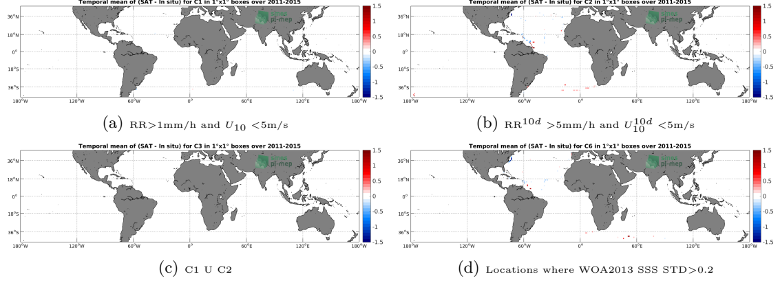
Figure 12: Temporal mean gridded over spatial boxes of size 1^\circ \times 1^\circ of \Delta SSS (Aquarius-L4-IPRC-V5-WEEKLY - TSG-GOSUD-Sailing-ship) for 4 different subdatasets corresponding to: RR > 1\text{mm/h} and U_{10} < 5\text{m/s} (a), RR^{10d} > 5\text{mm/h} and U_{10}^{10d} < 5\text{m/s} (b), C1 U C2 (c), Locations where WOA2013 SSS STD > 0.2 (d).
