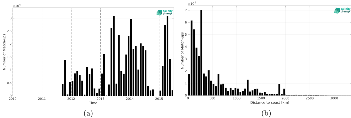
Figure 2: Number of match-ups between TSG (GOSUD-Research-vessel) and Aquarius SSS L4 OI v5 - Weekly (IPRC) SSS as a function of time (a) and as function of the distance to coast (b) over the Mid-Low Latitudes 45N-45S Pi-MEP region and for the full satellite product period.
