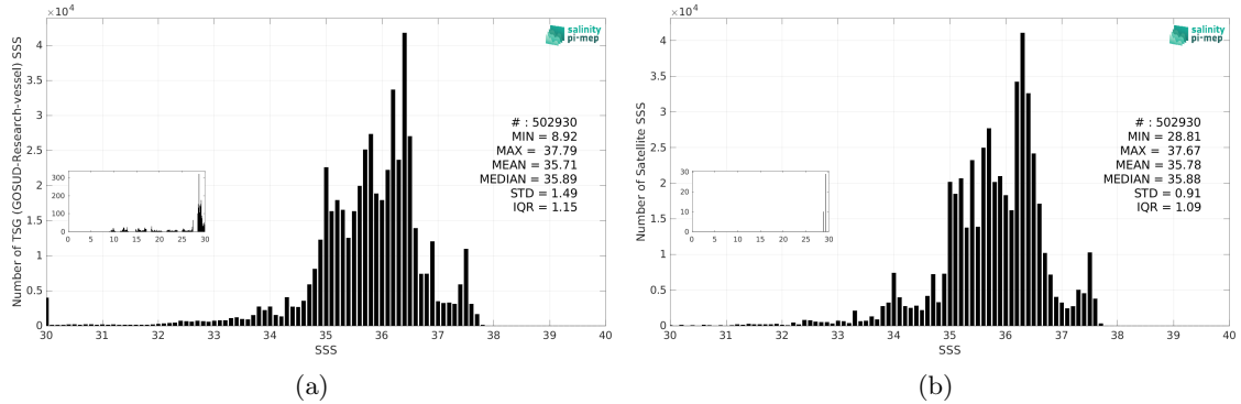
Figure 3: Histograms of SSS from TSG (GOSUD-Research-vessel) (a) and Aquarius SSS L4 OI v5 - Weekly (IPRC) (b) considering all match-up pairs per bins of 0.1 over the Mid-Low Latitudes 45N-45S Pi-MEP region and for the full satellite product period.
