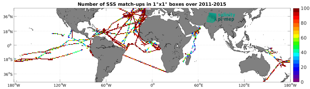
Figure 5: Number of SSS match-ups between TSG (GOSUD-Research-vessel) SSS and the Aquarius SSS L4 OI v5 - Weekly (IPRC) SSS product for the Mid-Low Latitudes 45N-45S Pi-MEP region over 1^{\circ} \times 1^{\circ} boxes and for the full satellite product period.
