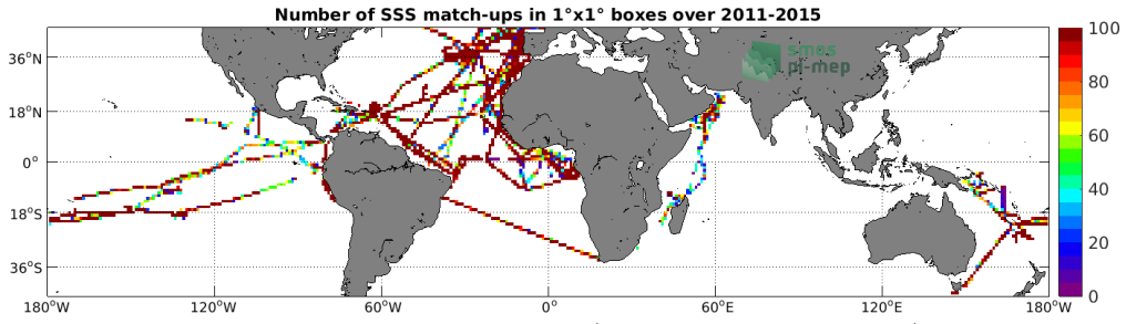
Figure 4: Number of SSS match-ups between TSG (GOSUD-Research-vessel) SSS and the Aquarius SSS L4 OI v5 - Weekly (IPRC) SSS product for the Mid-Low Latitudes 45N-45S Pi-MEP region over 1^\circ \times 1^\circ boxes and for the full satellite product period.
