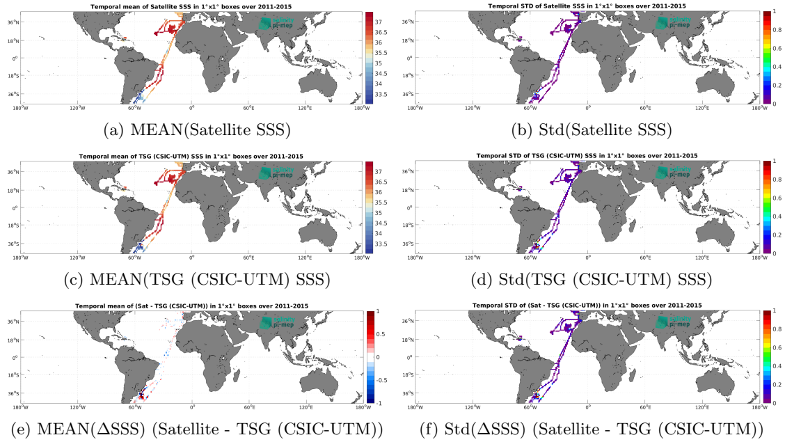
Figure 7: Temporal mean (left) and Std (right) of SSS from Aquarius SSS L4 OI v5 - Weekly (IPRC) (top), TSG (CSIC-UTM) (middle), and of \Delta SSS (Satellite - TSG (CSIC-UTM)). Only match-up pairs are used to generate these maps.
