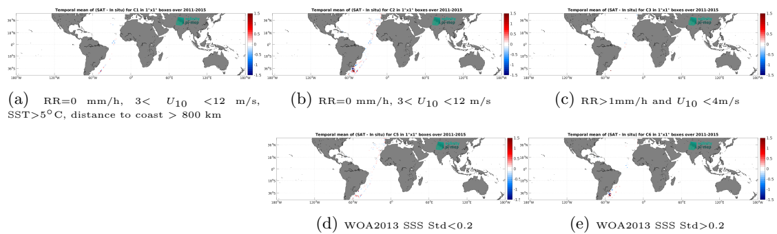
Figure 14: Temporal mean gridded over spatial boxes of size 1^\circ \times 1^\circ of \Delta\text{SSS} (Aquarius SSS L4 OI v5 - Weekly (IPRC) - TSG (CSIC-UTM)) for 5 different subdatasets corresponding to: RR=0 mm/h, 3 < U_{10} < 12 m/s, SST > 5°C, distance to coast > 800 km (a), RR=0 mm/h, 3 < U_{10} < 12 m/s (b), RR > 1mm/h and U_{10} < 4 m/s (c), WOA2013 SSS Std < 0.2 (d), WOA2013 SSS Std > 0.2 (e).
