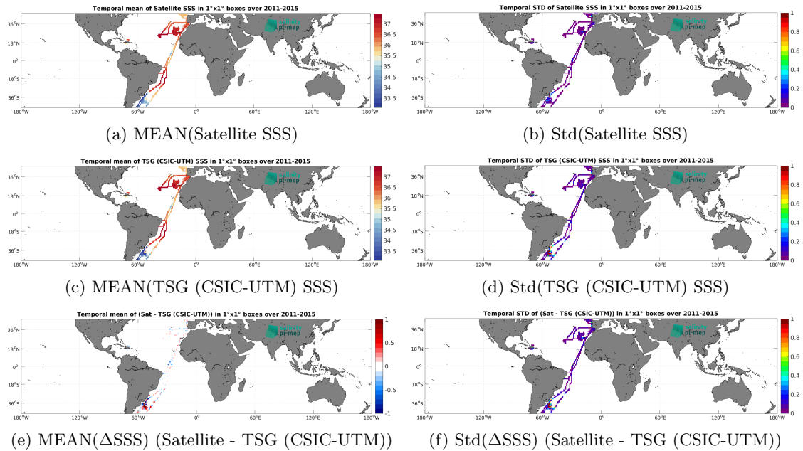
Figure 6: Temporal mean (left) and Std (right) of SSS from Aquarius SSS L4 OI v5 - Weekly (IPRC) (top), TSG (CSIC-UTM) (middle), and of \Delta SSS (Satellite - TSG (CSIC-UTM)). Only match-up pairs are used to generate these maps.
