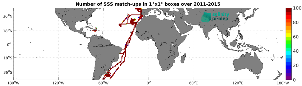
Figure 4: Number of SSS match-ups between TSG (CSIC-UTM) SSS and the Aquarius SSS L4 OI v5 - Weekly (IPRC) SSS product for the Mid-Low Latitudes 45N-45S Pi-MEP region over 1^\circ \times 1^\circ boxes and for the full satellite product period.
