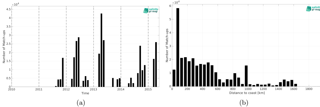
Figure 1: Number of match-ups between TSG (CSIC-UTM) and Aquarius SSS L4 OI v5 - Weekly (IPRC) SSS as a function of time (a) and as function of the distance to coast (b) over the Mid-Low Latitudes 45N-45S Pi-MEP region and for the full satellite product period.
