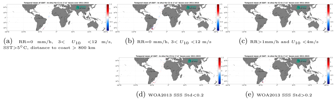
Figure 12: Temporal mean gridded over spatial boxes of size 1^\circ \times 1^\circ of \Delta SSS (Aquarius SSS L4 OI v5 - Weekly (IPRC) - TSG (CSIC-UTM)) for 5 different subdatasets corresponding to: RR=0 mm/h, 3 < U_{10} < 12 m/s, SST > 5^\circ\text{C} , distance to coast > 800 km (a), RR=0 mm/h, 3 < U_{10} < 12 m/s (b), RR > 1 mm/h and U_{10} < 4 m/s (c), WOA2013 SSS Std < 0.2 (d), WOA2013 SSS Std > 0.2 (e).
