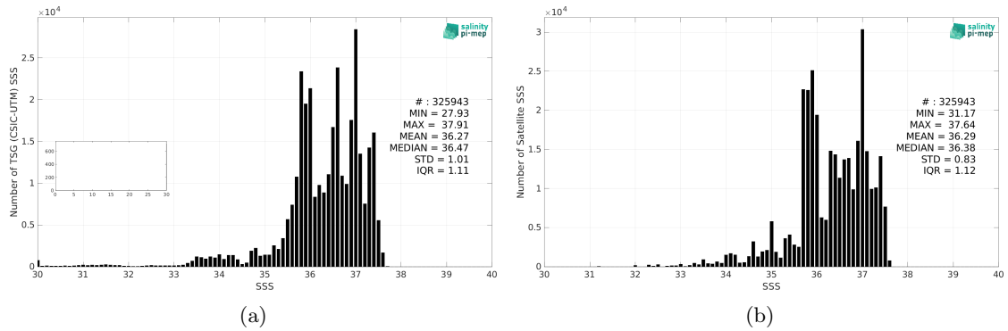
Figure 2: Histograms of SSS from TSG (CSIC-UTM) (a) and Aquarius SSS L4 OI v5 - Weekly (IPRC) (b) considering all match-up pairs per bins of 0.1 over the Mid-Low Latitudes 45N-45S Pi-MEP region and for the full satellite product period.
