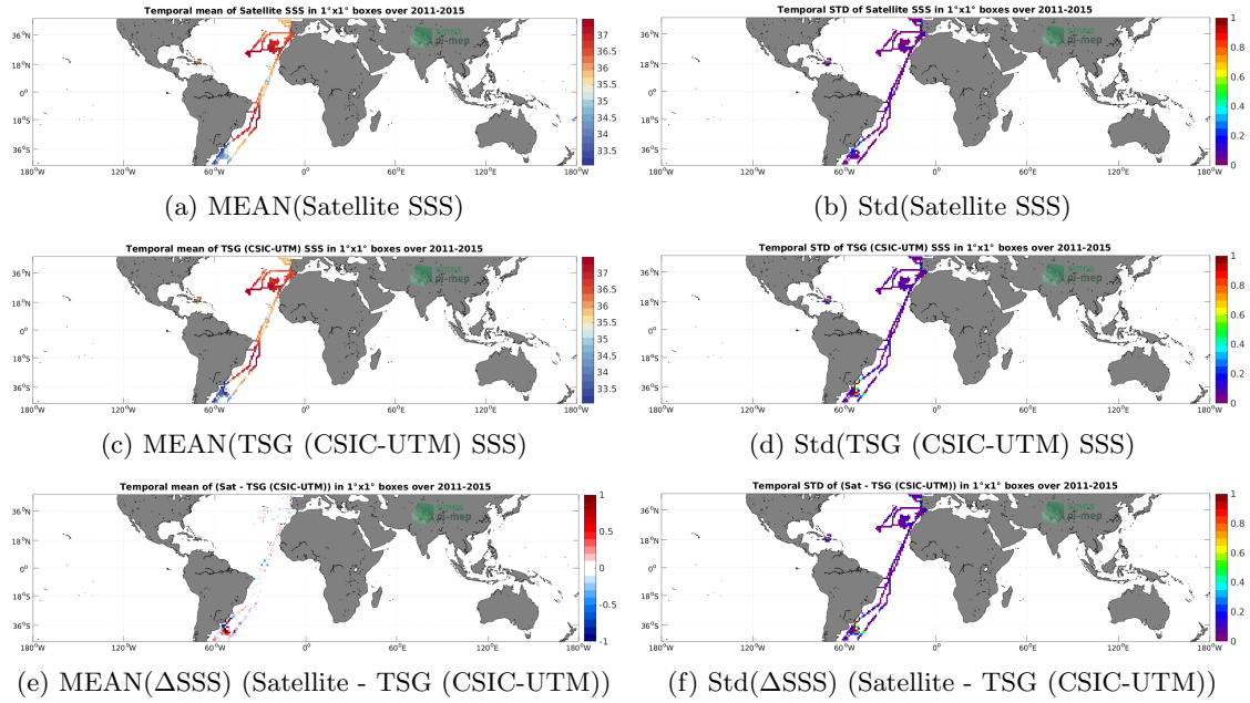
Figure 6: Temporal mean (left) and Std (right) of SSS from Aquarius SSS L4 OI v5 - Weekly (IPRC) (top), TSG (CSIC-UTM) (middle), and of \Delta SSS (Satellite - TSG (CSIC-UTM)). Only match-up pairs are used to generate these maps.
