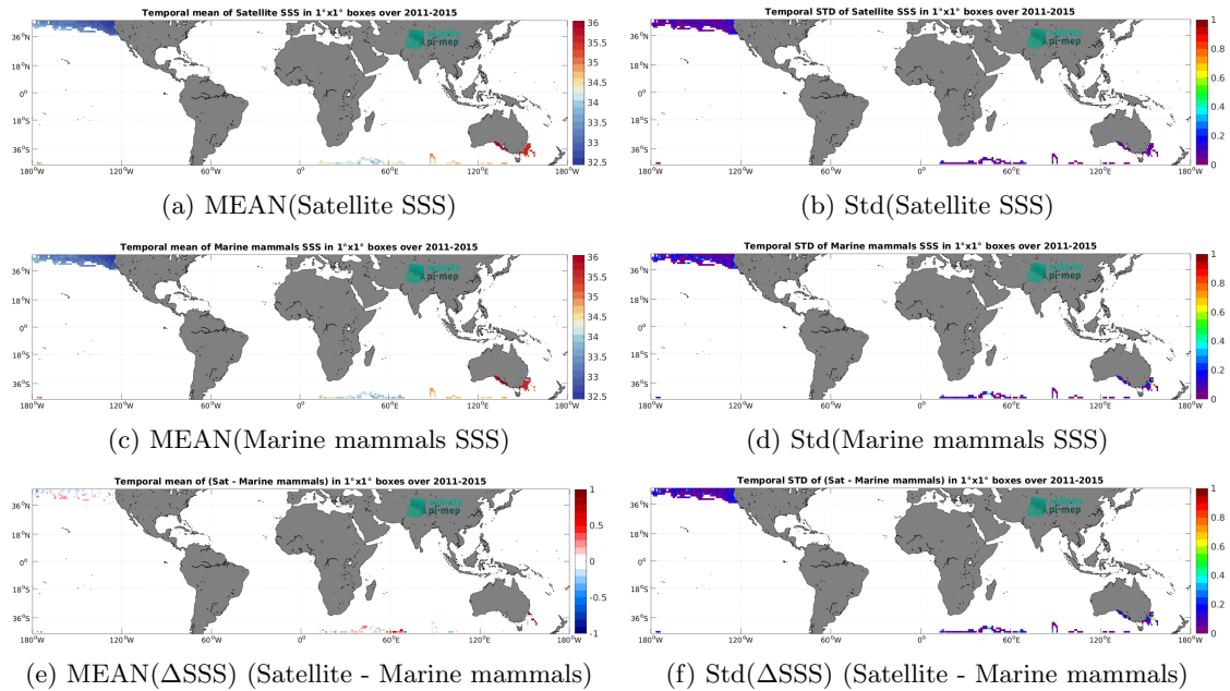
Figure 7: Temporal mean (left) and Std (right) of SSS from Aquarius SSS L4 OI v5 - Weekly (IPRC) (top), Marine mammals (middle), and of \Delta SSS (Satellite - Marine mammals). Only match-up pairs are used to generate these maps.
