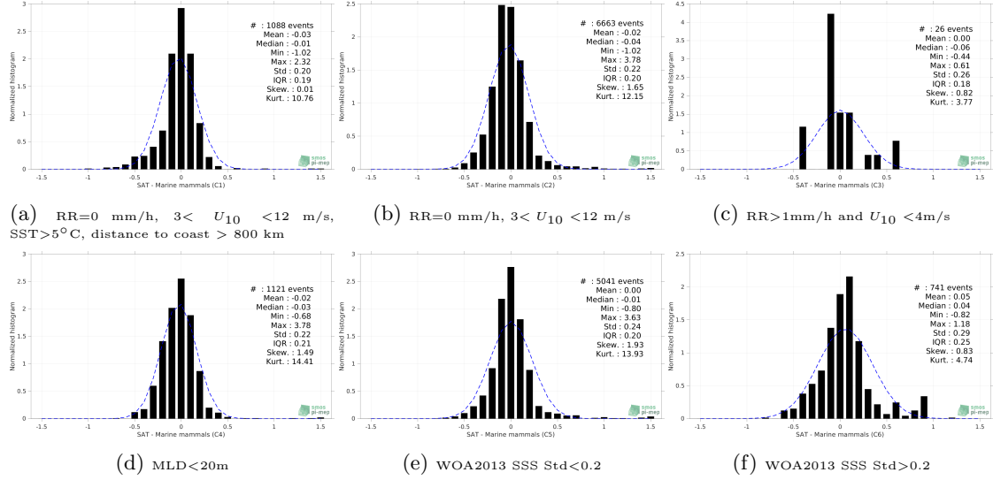
Figure 13: Normalized histogram of \Delta SSS (Aquarius SSS L4 OI v5 - Weekly (IPRC) - Marine mammals) for 6 different subdatasets corresponding to: RR=0 mm/h, 3 < U_{10} < 12 m/s, SST>5°C, distance to coast > 800 km (a), RR=0 mm/h, 3 < U_{10} < 12 m/s (b), RR>1mm/h and U_{10} < 4 m/s (c), MLD<20m (d), WOA2013 SSS Std<0.2 (e), WOA2013 SSS Std>0.2 (f).
