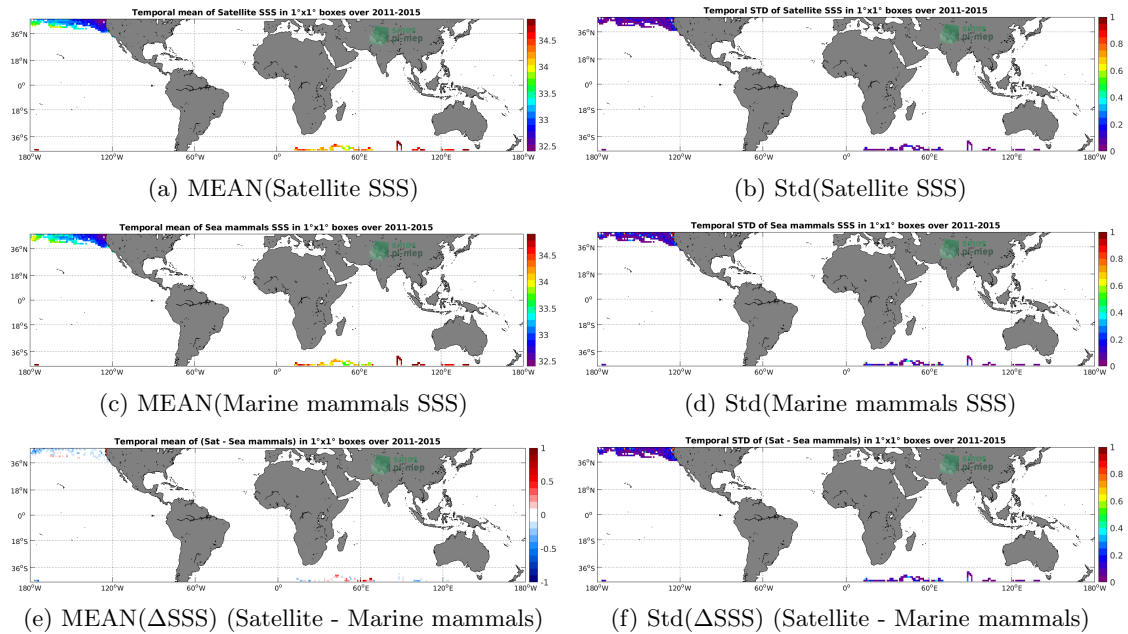
Figure 6: Temporal mean (left) and Std (right) of SSS from Aquarius SSS L4 OI v5 - Weekly (IPRC) (top), Marine mammals (middle), and of \Delta SSS (Satellite - Marine mammals). Only match-up pairs are used to generate these maps.
