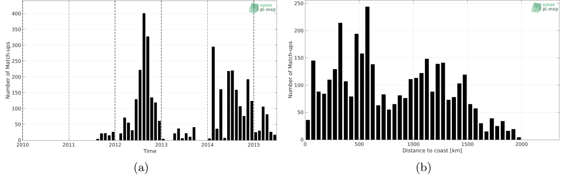
Figure 1: Number of match-ups between Sea mammals and Aquarius SSS L4 OI v5 - Weekly (IPRC) SSS as a function of time (a) and as function of the distance to coast (b) over the Mid-Low Latitudes 45N-45S Pi-MEP region and for the full satellite product period.
