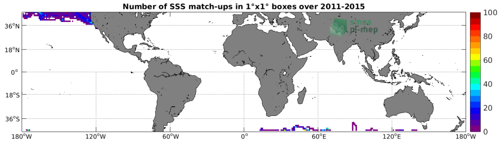
Figure 4: Number of SSS match-ups between Sea mammals SSS and the Aquarius SSS L4 OI v5 - Weekly (IPRC) SSS product for the Mid-Low Latitudes 45N-45S Pi-MEP region over 1°x1° boxes and for the full satellite product period.
