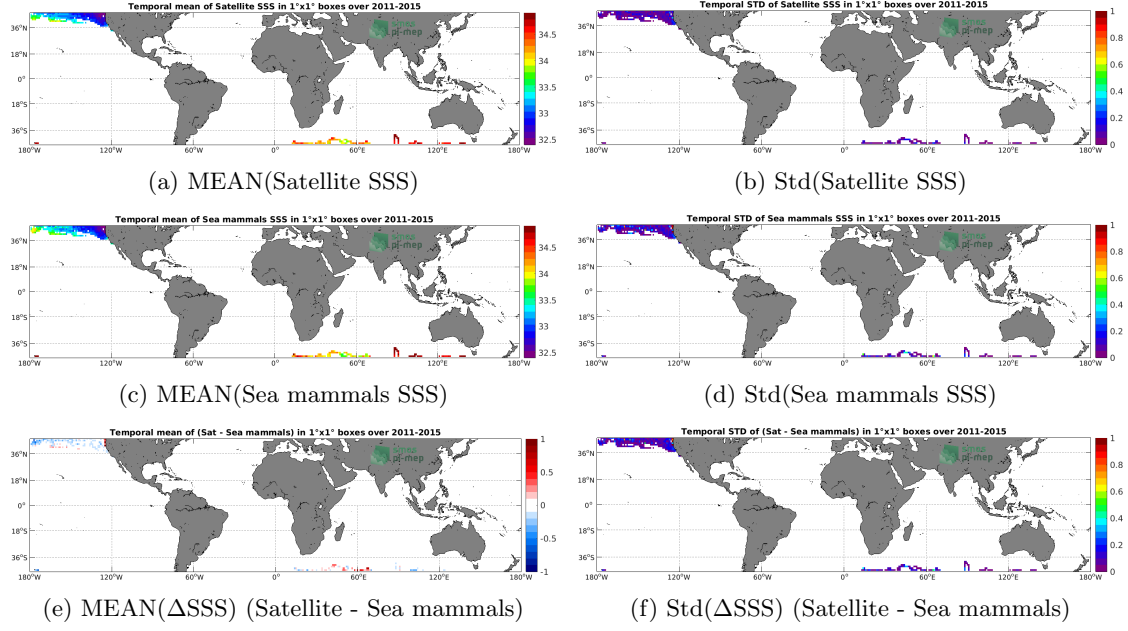
Figure 6: Temporal mean (left) and Std (right) of SSS from Aquarius SSS L4 OI v5 - Weekly (IPRC) (top), Sea mammals (middle), and of \Delta SSS (Satellite - Sea mammals). Only match-up pairs are used to generate these maps.
