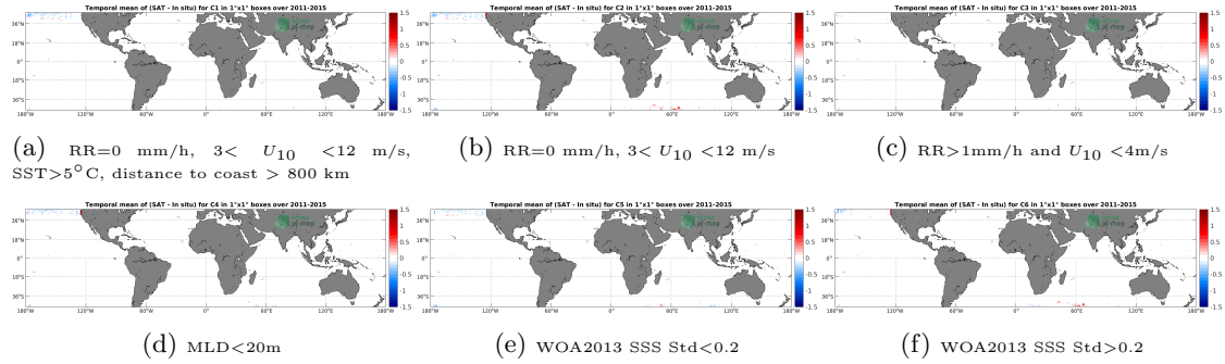
Figure 12: Temporal mean gridded over spatial boxes of size 1^\circ \times 1^\circ of \Delta SSS (Aquarius SSS L4 OI v5 - Weekly (IPRC) - Sea mammals) for 6 different subdatasets corresponding to: RR=0 mm/h, 3 < U_{10} < 12 m/s, SST > 5^\circ C , distance to coast > 800 km (a), RR=0 mm/h, 3 < U_{10} < 12 m/s (b), RR > 1 mm/h and U_{10} < 4 m/s (c), MLD < 20 m (d), WOA2013 SSS Std < 0.2 (e), WOA2013 SSS Std > 0.2 (f).
