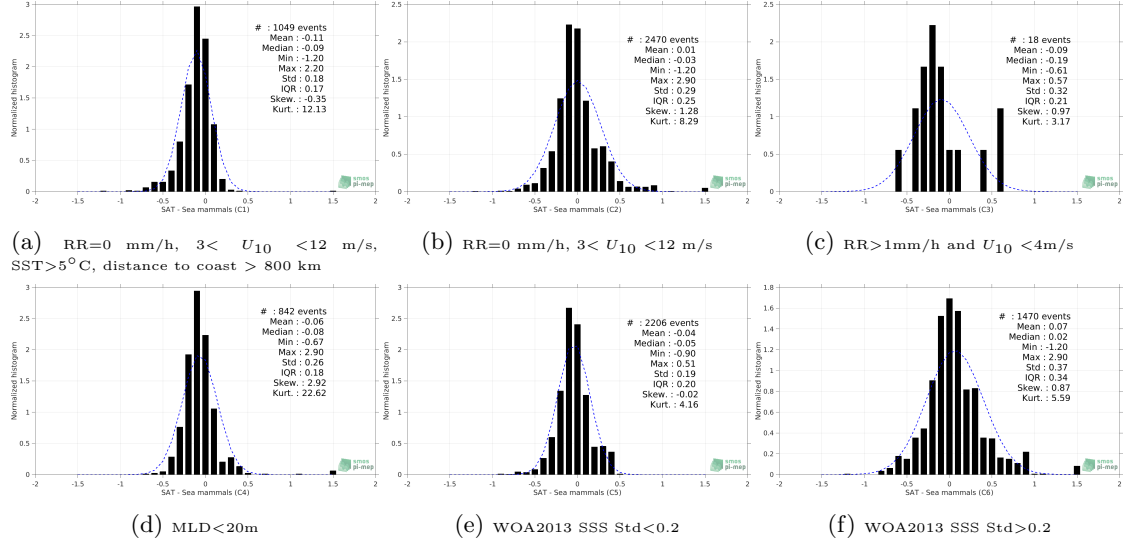
Figure 13: Normalized histogram of \Delta SSS (Aquarius SSS L4 OI v5 - Weekly (IPRC) - Sea mammals) for 6 different subdatasets corresponding to: RR=0 mm/h, 3 < U_{10} < 12 m/s, SST>5°C, distance to coast > 800 km (a), RR=0 mm/h, 3 < U_{10} < 12 m/s (b), RR>1mm/h and U_{10} < 4 m/s (c), MLD<20m (d), WOA2013 SSS Std<0.2 (e), WOA2013 SSS Std>0.2 (f).
