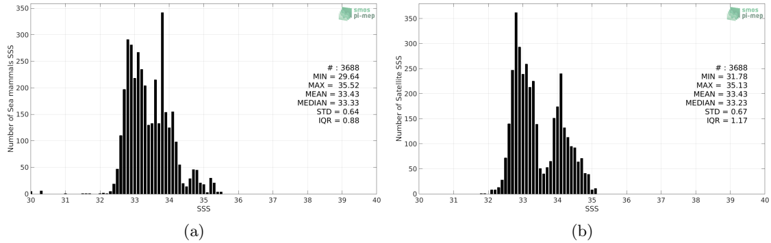
Figure 2: Histograms of SSS from Sea mammals (a) and Aquarius SSS L4 OI v5 - Weekly (IPRC) (b) considering all match-up pairs per bins of 0.1 over the Mid-Low Latitudes 45N-45S Pi-MEP region and for the full satellite product period.
