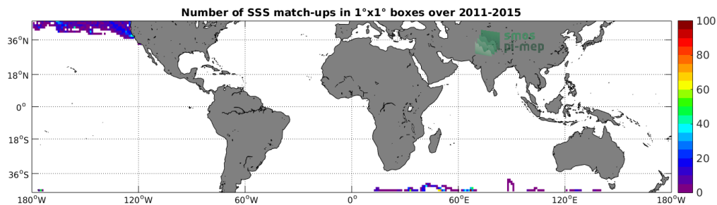
Figure 4: Number of SSS match-ups between Sea mammals SSS and the Aquarius-L4-IPRC-V5-WEEKLY SSS product for the Mid-Low Latitudes 45N-45S Pi-MEP region over 1^\circ \times 1^\circ boxes and for the full satellite product period.
