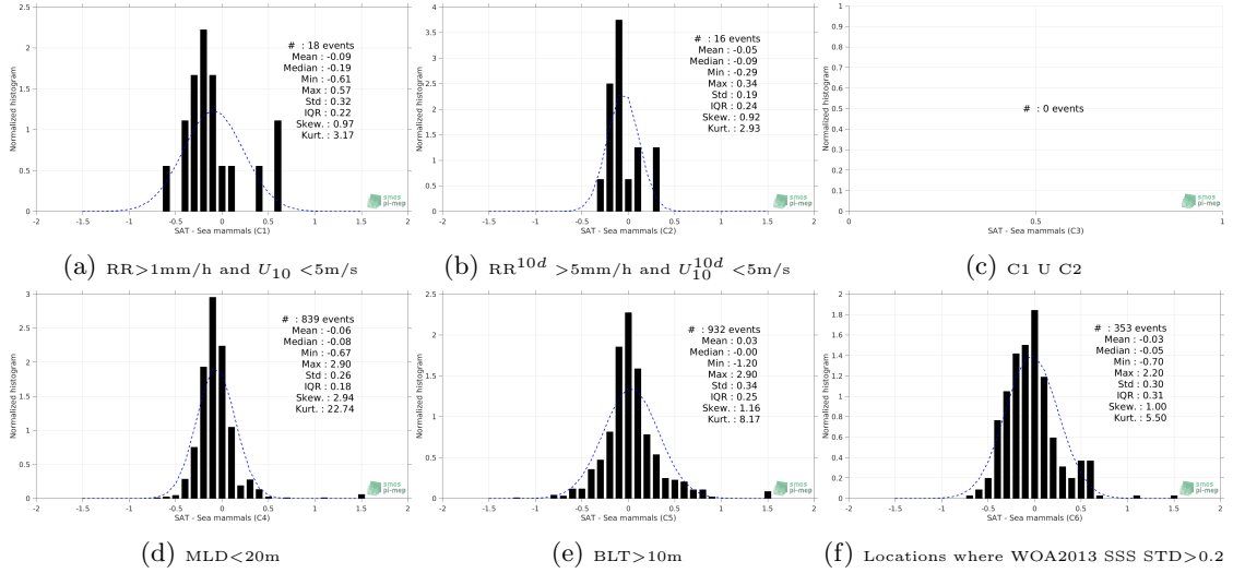
Figure 13: Normalized histogram of \Delta\text{SSS} (Aquarius-L4-IPRC-V5-WEEKLY - Sea mammals) for 6 different subdatasets corresponding to: \text{RR}>1\text{mm/h} and U_{10}<5\text{m/s} (a), \text{RR}^{10d}>5\text{mm/h} and U_{10}^{10d}<5\text{m/s} (b), C1 U C2 (c), \text{MLD}<20\text{m} (d), \text{BLT}>10\text{m} (e), Locations where WOA2013 SSS \text{STD}>0.2 (f).
