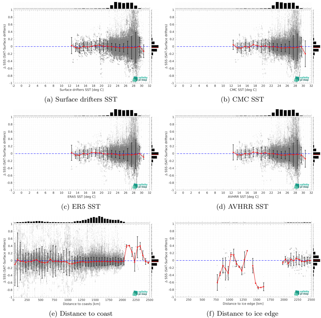
Figure 12: \Delta \text{SSS} (Satellite - Surface drifters) sorted as function of Surface drifters SST values (a), CMC SST (b), ERA5 SST (c), AVHRR SST (d), distance to coast (e) and distance to ice edge (f). In all plots the median and Std of \Delta \text{SSS} for each bin is indicated by the red curves and black vertical thick bars ( \pm 1 \text{ Std} ). Link to a similar figure sorted as function of Sea ice fraction.
