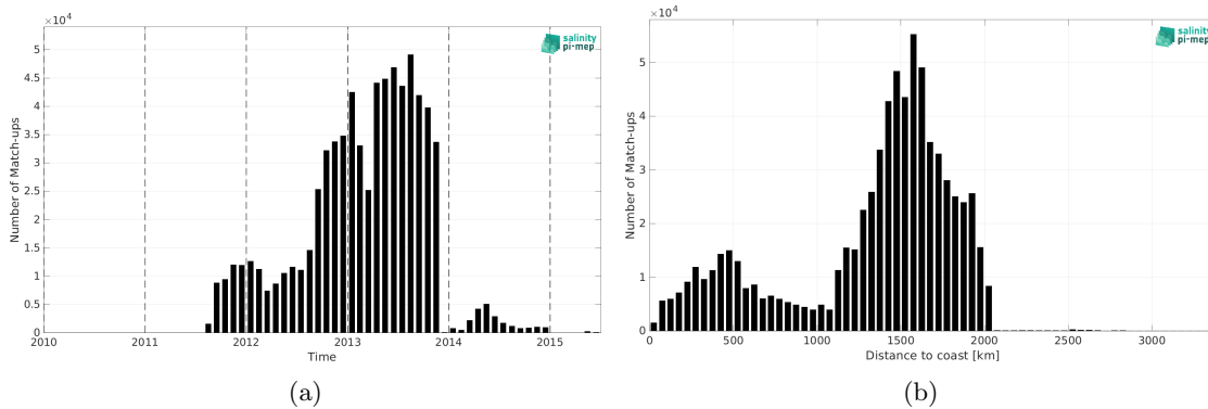
Figure 2: Number of match-ups between Surface drifters and Aquarius SSS L4 OI v5 - Weekly (IPRC) SSS as a function of time (a) and as function of the distance to coast (b) over the Mid-Low Latitudes 45N-45S Pi-MEP region and for the full satellite product period.
