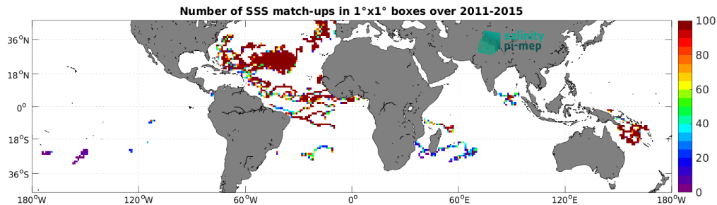
Figure 4: Number of SSS match-ups between Surface drifters SSS and the Aquarius SSS L4 OI v5 - Weekly (IPRC) SSS product for the Mid-Low Latitudes 45N-45S Pi-MEP region over 1^\circ \times 1^\circ boxes and for the full satellite product period.
