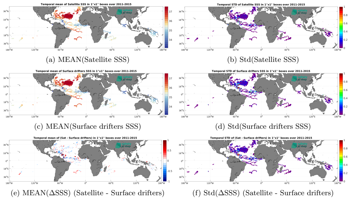
Figure 6: Temporal mean (left) and Std (right) of SSS from Aquarius SSS L4 OI v5 - Weekly (IPRC) (top), Surface drifters (middle), and of \Delta SSS (Satellite - Surface drifters). Only match-up pairs are used to generate these maps.
