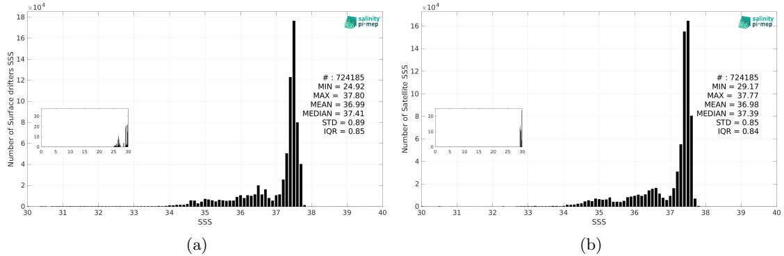
Figure 3: Histograms of SSS from Surface drifters (a) and Aquarius SSS L4 OI v5 - Weekly (IPRC) (b) considering all match-up pairs per bins of 0.1 over the Mid-Low Latitudes 45N-45S Pi-MEP region and for the full satellite product period.
