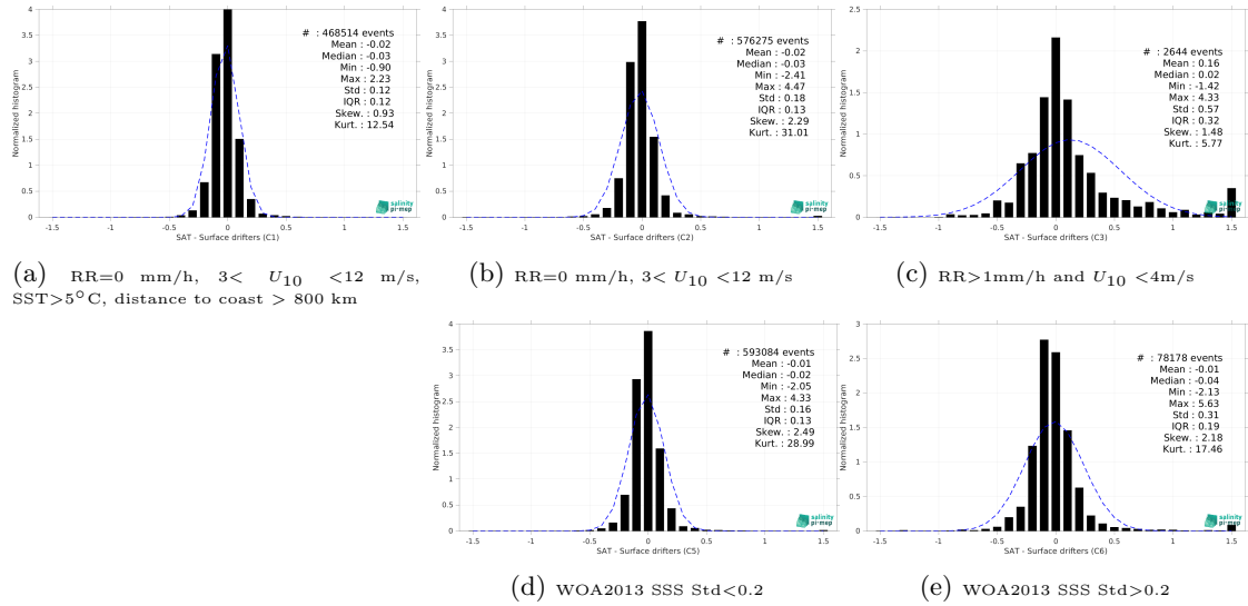
Figure 14: Normalized histogram of \Delta\text{SSS} (Aquarius SSS L4 OI v5 - Weekly (IPRC) - Surface drifters) for 5 different subdatasets corresponding to: RR=0 mm/h, 3 < U_{10} < 12 m/s, SST>5°C, distance to coast > 800 km (a), RR=0 mm/h, 3 < U_{10} < 12 m/s (b), RR>1mm/h and U_{10} < 4 m/s (c), WOA2013 SSS Std<0.2 (d), WOA2013 SSS Std>0.2 (e).
