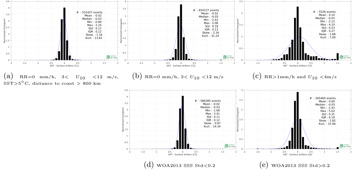
Figure 12: Normalized histogram of \Delta SSS (Aquarius SSS L4 OI v5 - Weekly (IPRC) - Surface drifters) for 5 different subdatasets corresponding to: RR=0 mm/h, 3 < U_{10} < 12 m/s, SST > 5^\circ C , distance to coast > 800 km (a), RR=0 mm/h, 3 < U_{10} < 12 m/s (b), RR > 1 mm/h and U_{10} < 4 m/s (c), WOA2013 SSS Std < 0.2 (d), WOA2013 SSS Std > 0.2 (e).
