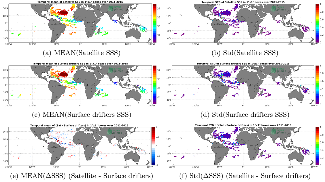
Figure 5: Temporal mean (left) and Std (right) of SSS from Aquarius SSS L4 OI v5 - Weekly (IPRC) (top), Surface drifters (middle), and of \Delta SSS (Satellite - Surface drifters). Only match-up pairs are used to generate these maps.
