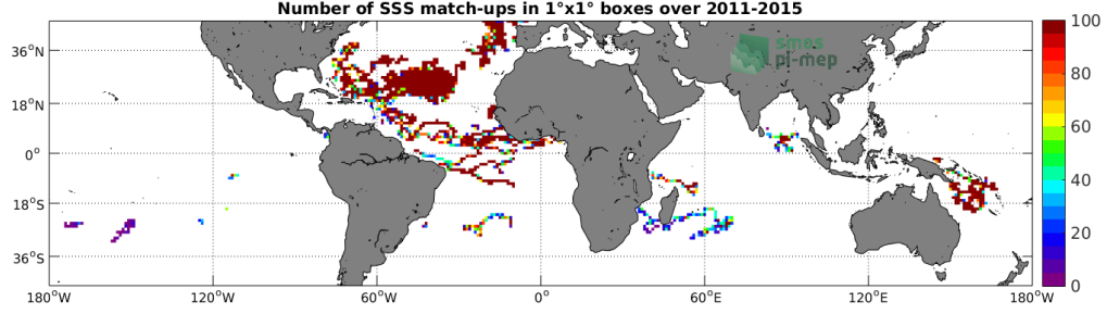
Figure 3: Number of SSS match-ups between Surface drifters SSS and the Aquarius-L4-IPRC-V5-WEEKLY SSS product for the Mid-Low Latitudes 45N-45S Pi-MEP region over 1^\circ \times 1^\circ boxes and for the full satellite product period.
