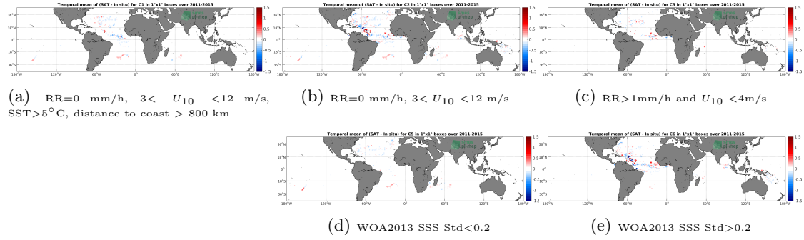
Figure 11: Temporal mean gridded over spatial boxes of size 1^\circ \times 1^\circ of \Delta SSS (Aquarius-L4-IPRC-V5-WEEKLY - Surface drifters) for 5 different subdatasets corresponding to:RR=0 mm/h, 3 < U_{10} < 12 m/s, SST >5^\circ\text{C} , distance to coast > 800 km (a), RR=0 mm/h, 3 < U_{10} < 12 m/s (b), RR >1 mm/h and U_{10} < 4 m/s (c), WOA2013 SSS Std <0.2 (d), WOA2013 SSS Std >0.2 (e).
