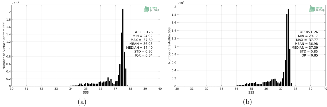
Figure 2: Histograms of SSS from Surface drifters (a) and Aquarius-L4-IPRC-V5-WEEKLY (b) considering all match-up pairs per bins of 0.1 over the Mid-Low Latitudes 45N-45S Pi-MEP region and for the full satellite product period.
