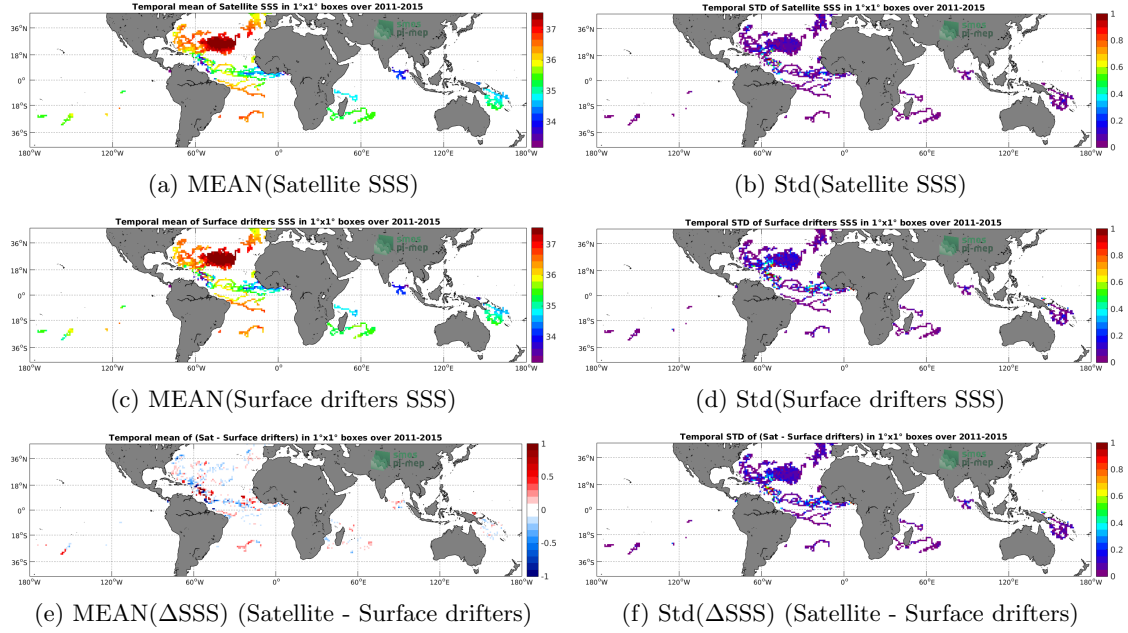
Figure 5: Temporal mean (left) and Std (right) of SSS from Aquarius-L4-IPRC-V5-WEEKLY (top), Surface drifters (middle), and of \Delta SSS (Satellite - Surface drifters). Only match-up pairs are used to generate these maps.
