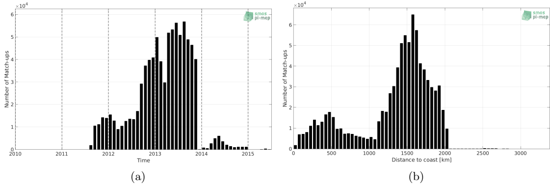
Figure 1: Number of match-ups between Surface drifters and Aquarius-L4-IPRC-V5-WEEKLY SSS as a function of time (a) and as function of the distance to coast (b) over the Mid-Low Latitudes 45N-45S Pi-MEP region and for the full satellite product period.
