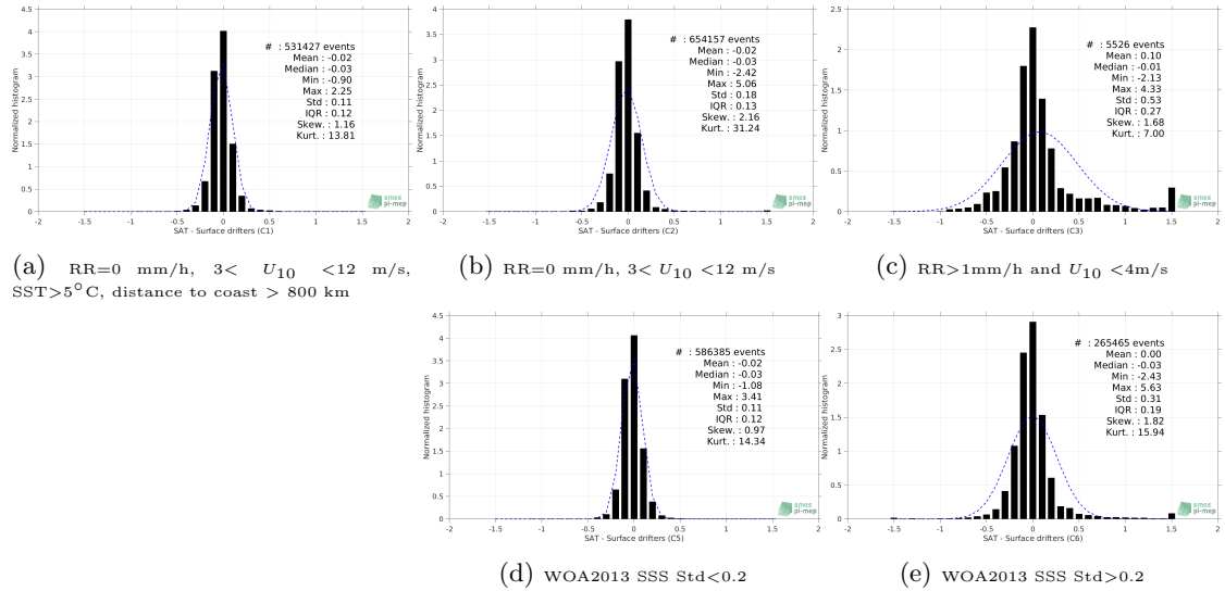
Figure 12: Normalized histogram of \Delta SSS (Aquarius-L4-IPRC-V5-WEEKLY - Surface drifters) for 5 different subdatasets corresponding to: RR=0 mm/h, 3 < U_{10} < 12 m/s, SST >5^\circ\text{C} , distance to coast > 800 km (a), RR=0 mm/h, 3 < U_{10} < 12 m/s (b), RR >1 mm/h and U_{10} < 4 m/s (c), WOA2013 SSS Std <0.2 (d), WOA2013 SSS Std >0.2 (e).
