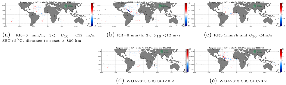
Figure 11: Temporal mean gridded over spatial boxes of size 1°x1° of \Delta SSS (Aquarius-L4-IPRC-V5-WEEKLY - Surface drifters) for 5 different subdatasets corresponding to: RR=0 mm/h, 3 < U_{10} < 12 m/s, SST > 5°C, distance to coast > 800 km (a), RR=0 mm/h, 3 < U_{10} < 12 m/s (b), RR > 1mm/h and U_{10} < 4m/s (c), WOA2013 SSS Std < 0.2 (d), WOA2013 SSS Std > 0.2 (e).
