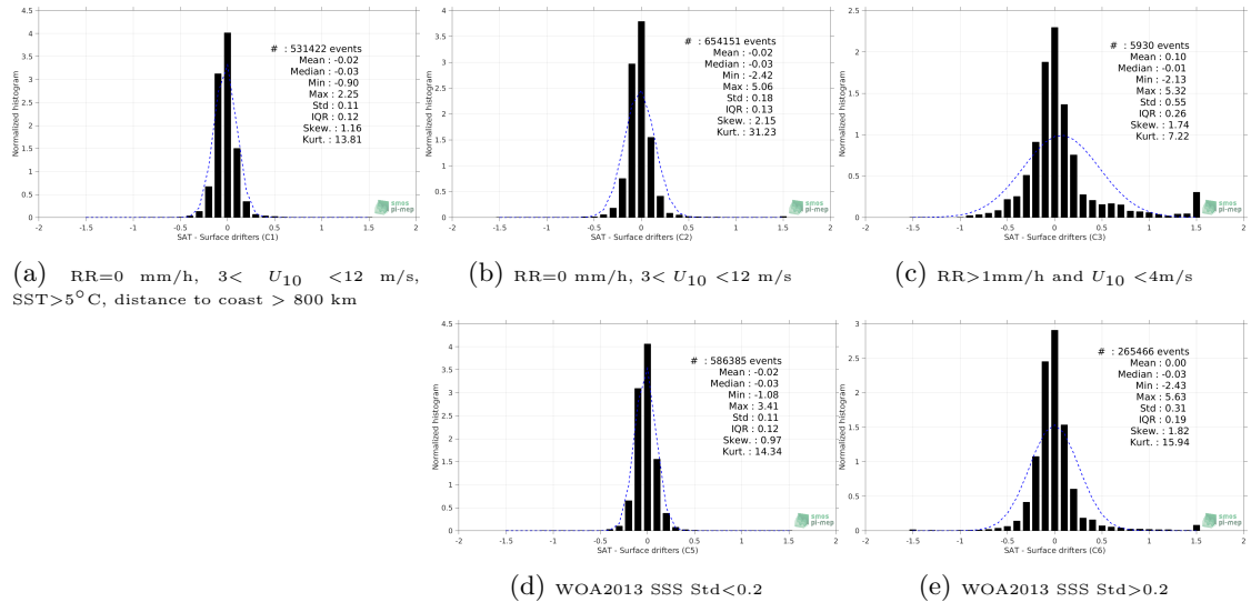
Figure 12: Normalized histogram of \Delta SSS (Aquarius-L4-IPRC-V5-WEEKLY - Surface drifters) for 5 different subdatasets corresponding to: RR=0 mm/h, 3 < U_{10} < 12 m/s, SST >5^\circ C, distance to coast > 800 km (a), RR=0 mm/h, 3 < U_{10} < 12 m/s (b), RR >1 mm/h and U_{10} < 4 m/s (c), WOA2013 SSS Std <0.2 (d), WOA2013 SSS Std >0.2 (e).
