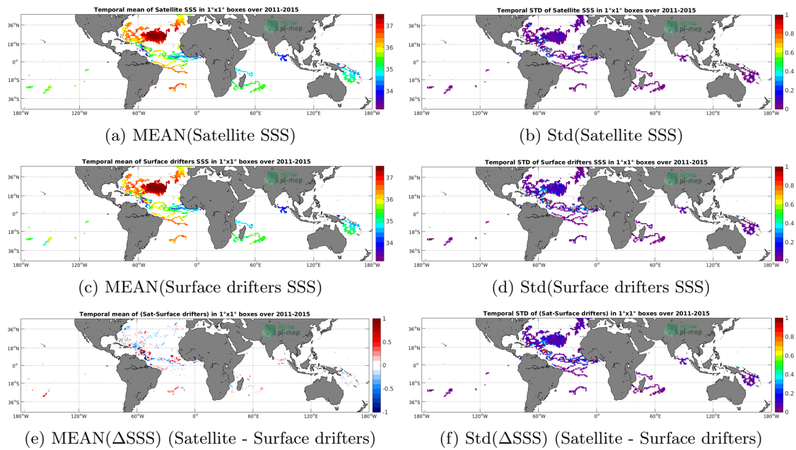
Figure 5: Temporal mean (left) and Std (right) of SSS from Aquarius-L4-IPRC-V5-WEEKLY (top), Surface drifters (middle), and of \Delta SSS (Satellite - Surface drifters). Only match-up pairs are used to generate these maps.
